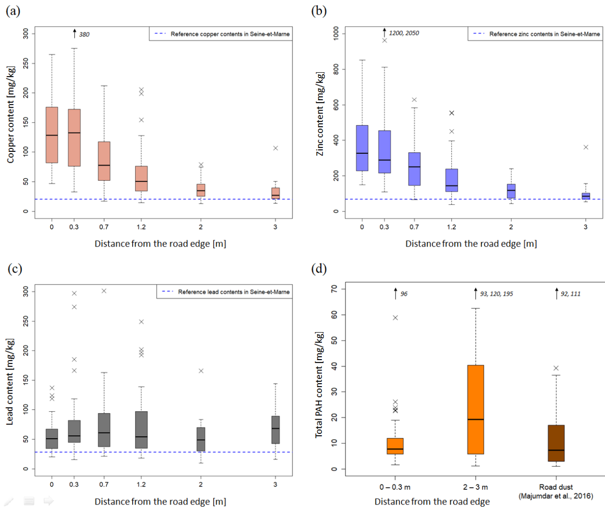
Fig. 4 – Concentrations of (a) copper, (b) zinc, (c) lead, and (d) \sum^{16} PAHs across all sites, as a function of the distance from the road. The bottom and top of each box correspond to the first and third quartiles, and the thick line represents the median value ( N = 40 ).
