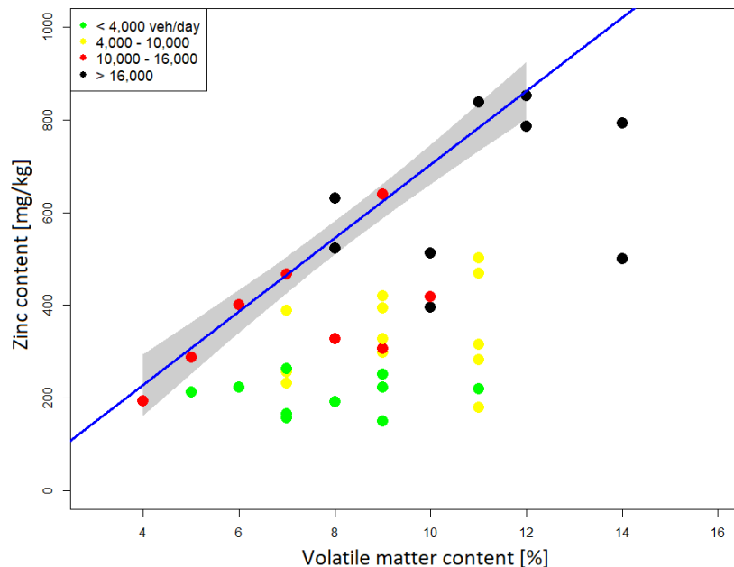
Fig. 7 – Relationship between volatile matter and zinc concentrations in the samples collected close to the road. The upper envelope of the data points (defined as the highest Zn concentration for each value of the volatile matter content) was modeled via a linear regression in the range 4\% \leq VM \leq 12\% (blue line, along with its 95% confidence interval).
