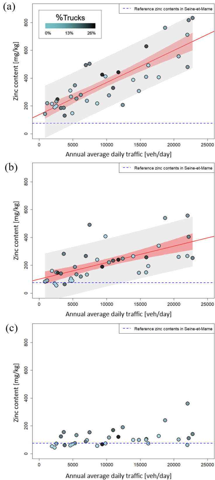
Fig. 6 – Relationship between the traffic characteristics (AADT on the horizontal axis and %Trucks represented as a color gradient) and the mean Zn concentrations (a) in the first 30 cm, (b) between 70 and 120 cm from the road, and (c) on the opposite side of each shoulder. The red and grey envelopes correspond respectively to the 95% confidence and prediction intervals of the regression.
