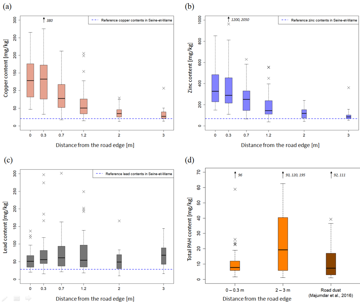
Fig. 4 – Concentrations of (a) copper, (b) zinc, (c) lead, and (d) \sum^{16} PAHs across all sites, as a function of the distance from the road. The bottom and top of each box correspond to the first and third quartiles, and the thick line represents the median value ( N = 40 ).
