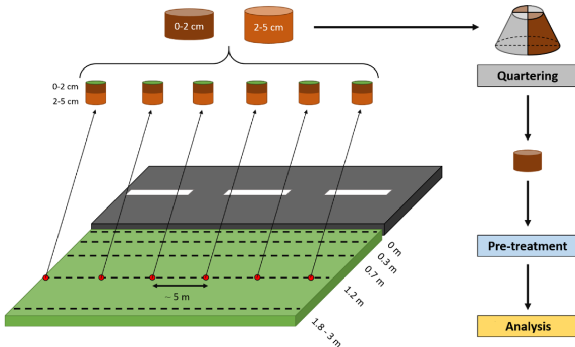
Fig. 3 – Schematic representation of the methodology for soil sampling and analysis (in the case of metals).
