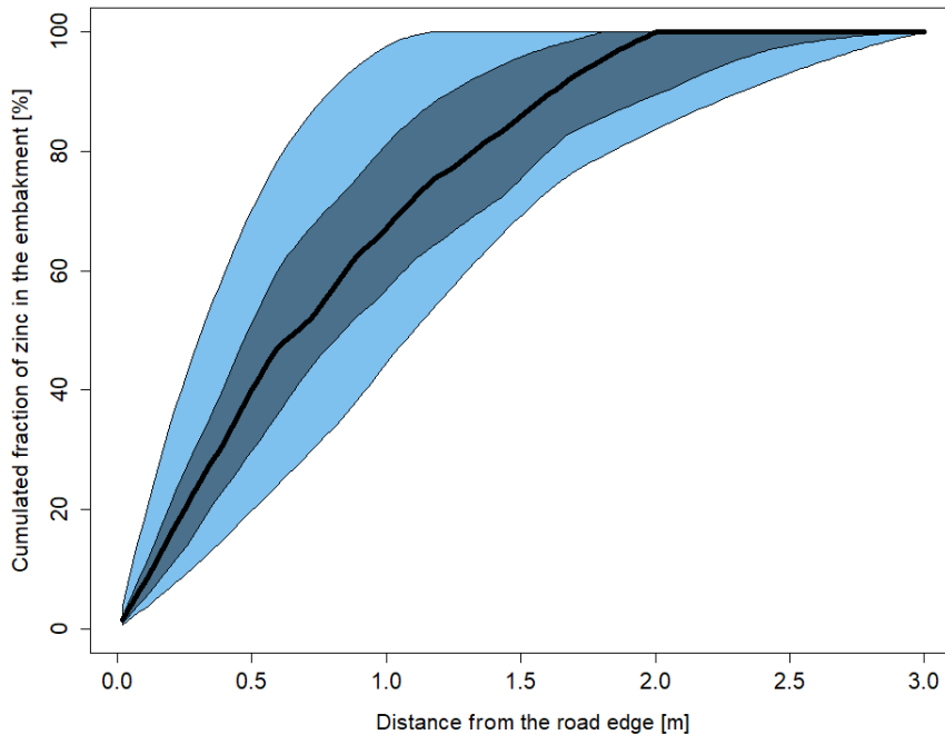
Fig. 8 – Fraction of zinc accumulated in the shoulder as a function of the distance from the road. The lines and envelopes represent statistics established from the 40 study sites: median accumulation (solid line), 1 st and 3 rd quartiles (dark envelope), 1 st and 9 th deciles (light envelope).
