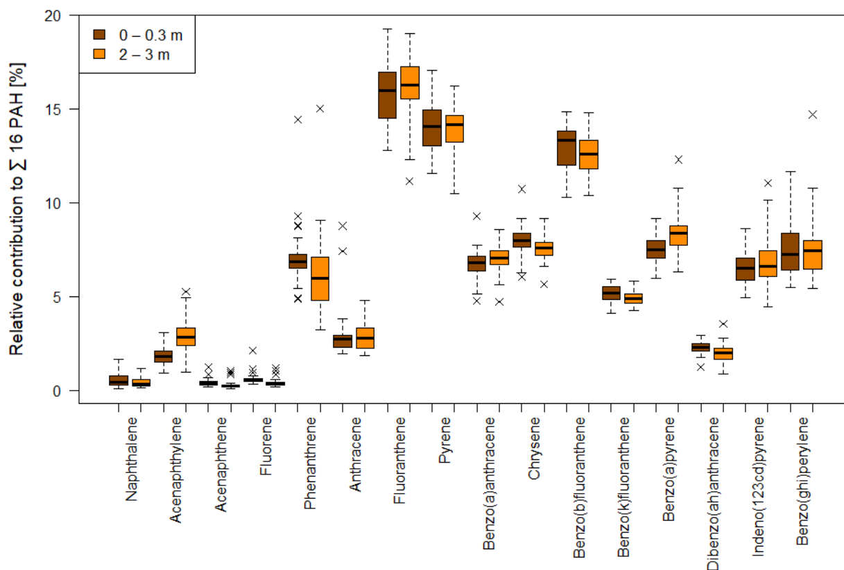
Fig. 5 – Relative contribution of each individual PAH to their total concentration, across all sites.
