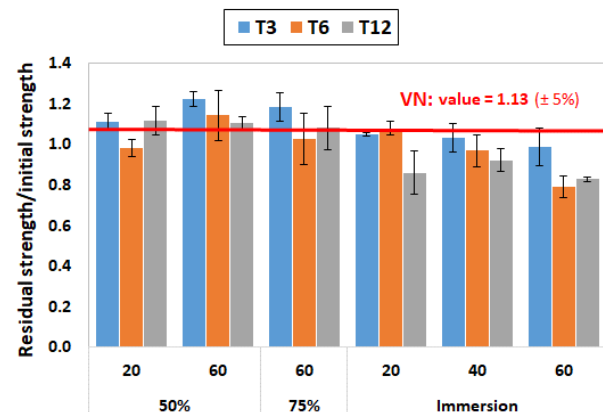
Fig. 4: Normalized residual strengths of specimens that were exposed to the various ageing conditions for periods up to 12 months. (T3, T6 and T12). The red line shows the value of the specimen exposed to weathering conditions (VN) for 12 months.
