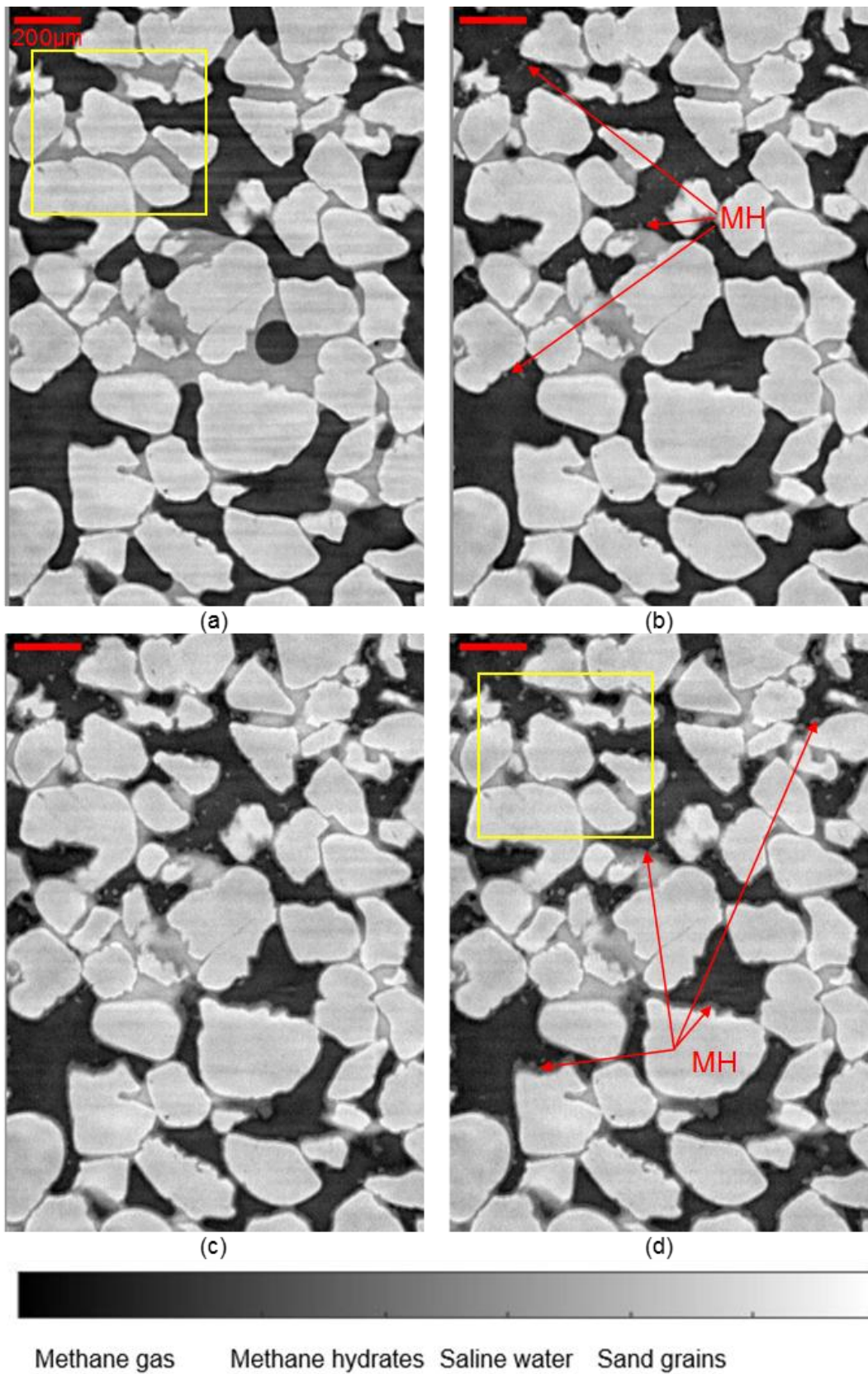
Figure 4. Vertical cross-section through Z0_HR: (a) t = 0 ; (b) t = 0.58 h; (b) t = 4 h; (c) t = 4.5 h.
