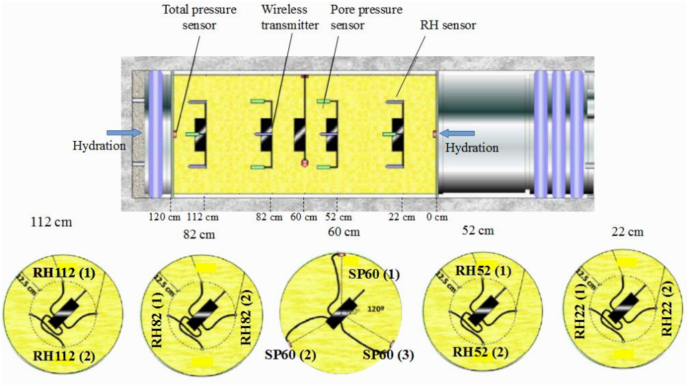
Fig. 2. Distribution of the relative humidity and swelling pressure sensors in the seal of SEALEX test.
