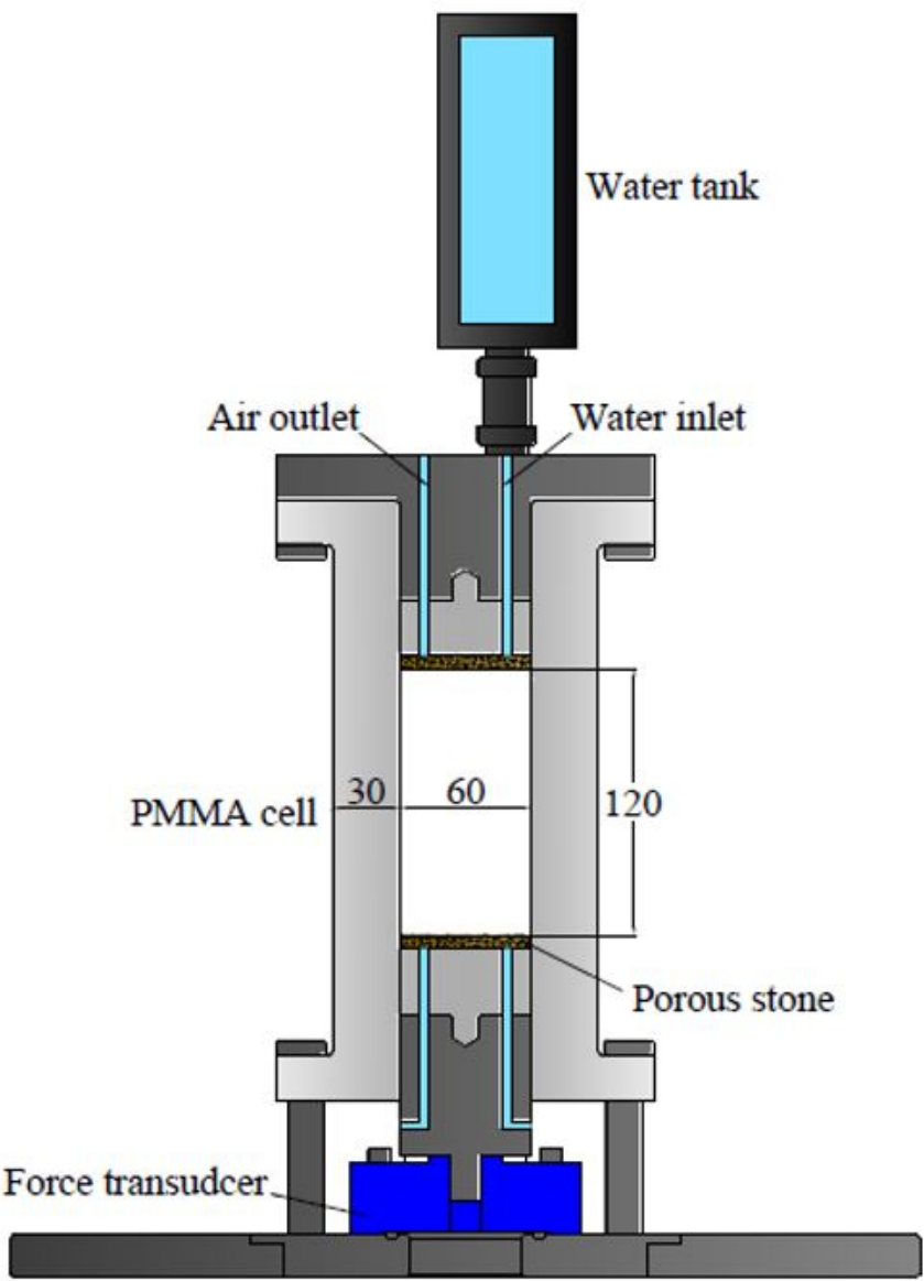
Fig. 4. Layout of the transparent PMMA cell. 175x242mm (72 x 72 DPI)
