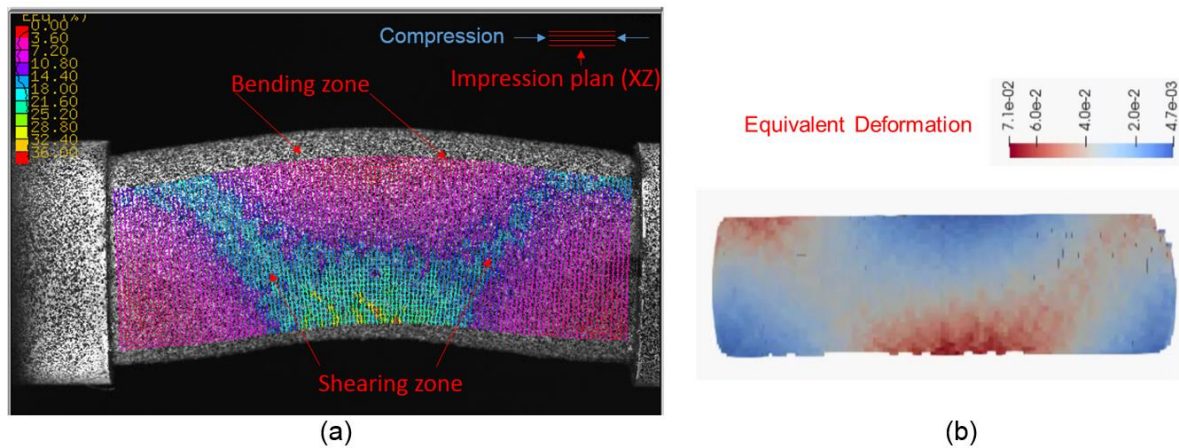
Figure 2: Equivalent strain field measured by 2D (a) and 3D image correlation (b).
