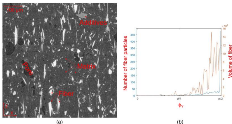
Figure 1: Cross-section along impression plane and fiber orientation distribution.
