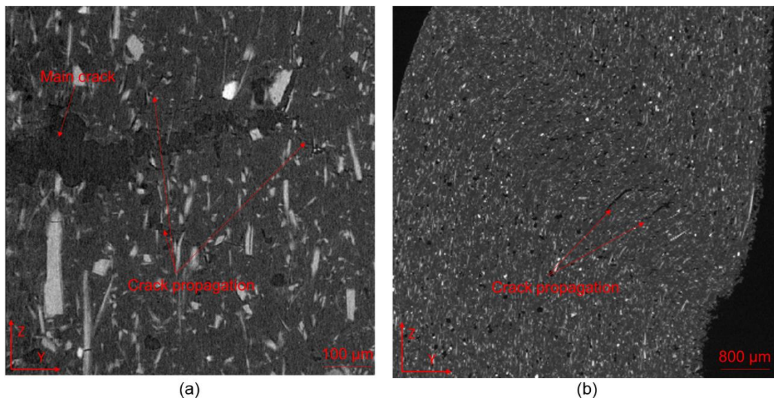
Figure 3: Cracks propagation in the bending zone (a) and in a shearing zone (b).
