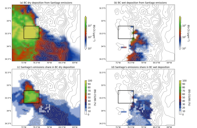
Figure 3: (a) BC dry deposition originating from Santiago's emissions, (b) same as (a) for wet deposition, (c) proportion of BC dry deposition originating from Santiago's emissions, (d) same as (c) for wet deposition. Total over July 2015 - CC5 simulation. The black box corresponds to the area where emissions are set to zero in the CS case. Grey contour levels are every 500 m starting from 1000 m a.s.l. White stars in (c) and (d) show the snow or ice-covered grid points considered in the continuation.
