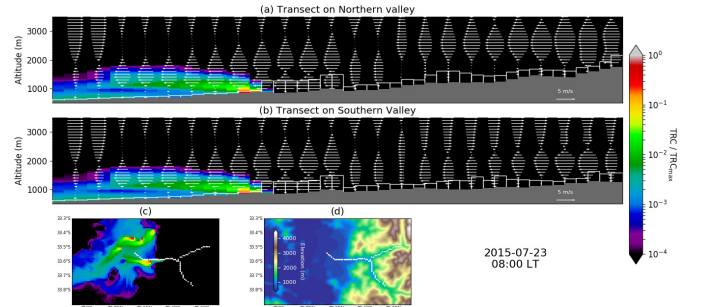
Figure A.4: Same as Figures A.2 and A.3 but on 23 July at 08:00 LT.
