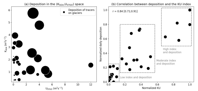
Figure 11: (a) Tracers dry deposition on the target area dependency on K_{SGA} and U_{STGO} . Circles areas are proportional to deposition. (b) Relationship between the normalized daily dry deposition and the normalized index KU/\max(KU) . The correlation is given with a 95% confidence interval.
