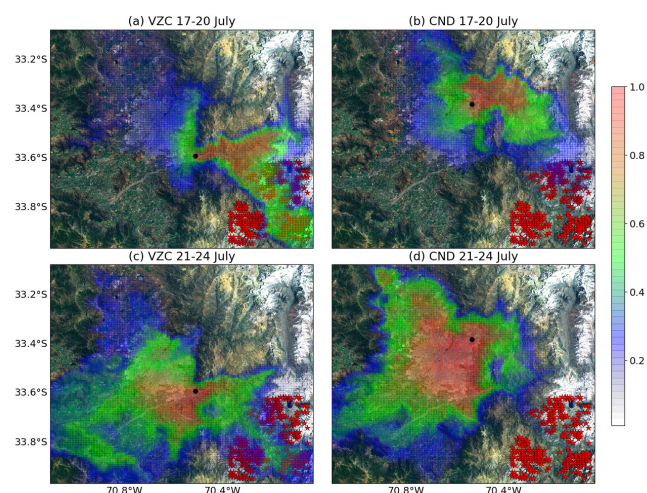
Figure 7: Frequency of tracer surface concentration above 0.2% of the maximum concentration at the source for two periods with distinct synoptic circulation (a) VZC for 17-20 July, (c) VZC for 21-24 July, (b) CND for 17-20 July, (d) CND for 21-24 July. Red stars show the target area, black dots the emission site. Map background layer: Imagery World 2D, ©2009 ESRI.
