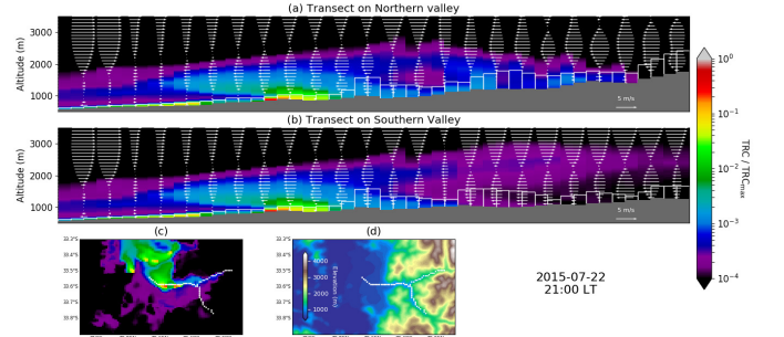
Figure A.3: Same as Figure A.2 but on 22 July at 21:00 LT.
