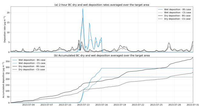
Figure 4: (a) Simulated time series of BC deposition over the target area in the BS case (solid line) and CS case (dashed line), (b) same as (a) but accumulated.
