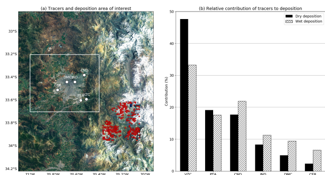
Figure 6: (a) Locations of considered passive tracers (white dots), and target area (red stars) influenced by emissions from Santiago (white box). Map background layer: Imagery World 2D, ©2009 ESRI (b) relative share of each tracer to dry and wet total deposition on the target area for July 2015.
