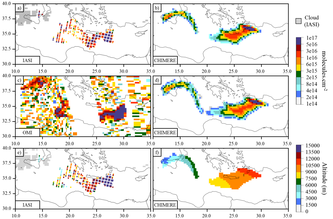
Figure 2. IASI \text{SO}_2 plume (a), OMI \text{SO}_2 plume (c), IASI and OMI soundings respectively for March 19 2012 06AM and 12AM UTC (3 and 4 in Table 3). CHIMERE \text{SO}_2 plume (b and d) in molecules.cm -2 corresponding to IASI and OMI soundings. IASI \text{SO}_2 altitude (e) and CHIMERE \text{SO}_2 maximum concentrations' altitude (f) in meters March 19 2012 06AM UTC. In this example, CHIMERE simulation WRFW-DL-20 is displayed. CHIMERE and OMI data are represented with OMI's 0.25^\circ \times 0.25^\circ resolution grid. Clouds are based on Advanced Very High Resolution Radiometer (AVHRR) data for IASI. Logscale is used to better visualized CHIMERE simulations, but values under 3\text{e}15 ( \sim 0.1\text{DU} ) are below satellite detection limits.
