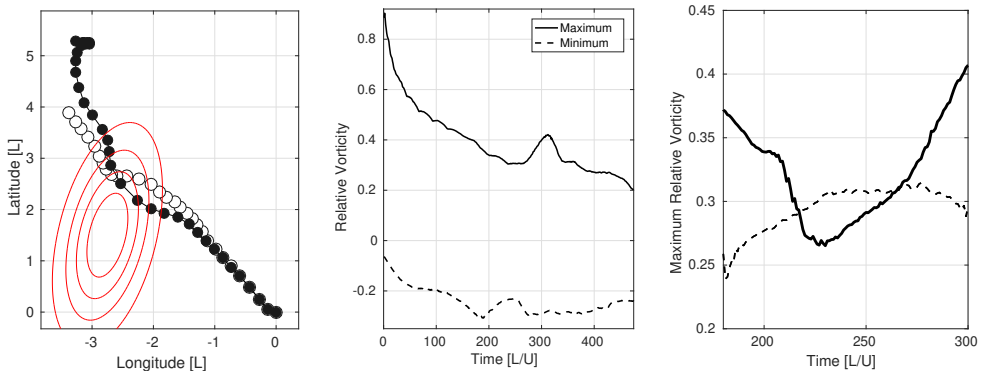
FIGURE 25. Left panel : trajectory of a TC - like vortex hitting the northern part of the “Taiwan” island with b_{max} = 0.2 (red contours) in the moist-convective environment (black circles) compared to that without topography. Time interval between the circles is 15 [L/U] . Middle panel : Corresponding evolution of the anticyclonic ( dashed ) and cyclonic ( solid ) peak relative vorticities. Right panel : Swap of the maximum of vorticity between the primary vortex ( solid ), and the secondary ( dashed ) terrain-induced cyclone.
