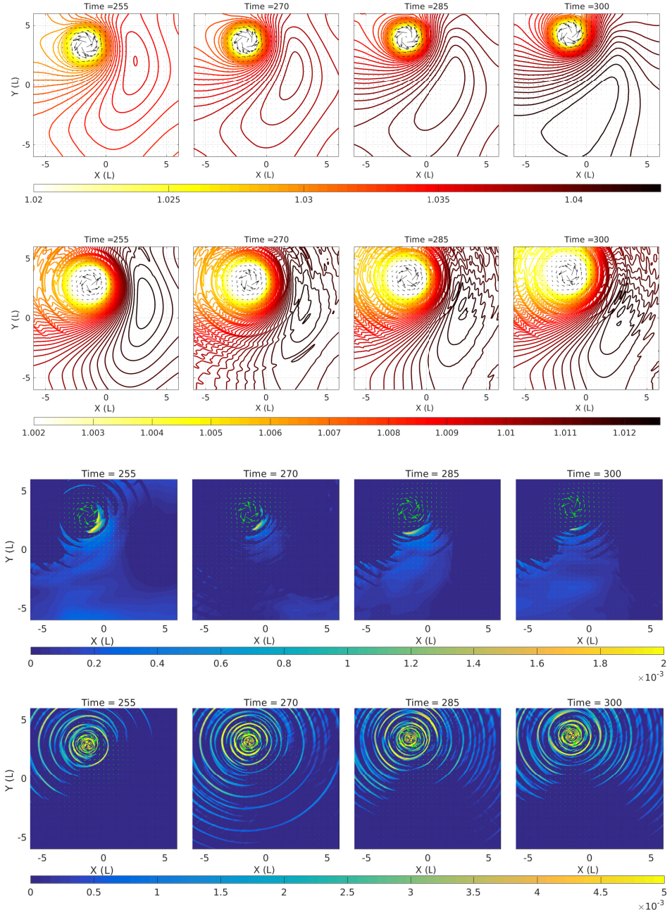
FIGURE 10. Snapshots of the isobars beyond the radius of maximum wind for the strongest vortex ( Ro = 19.3 ) of figure 9 in the “dry” (first row, ID : Dbis4 ) and moist-convective cases (second row, ID : MCbis4 ). Third row: Spatial distribution of condensation corresponding to the second row. Fourth row: Corresponding to the second row convection-coupled inertial gravity waves, as seen in the divergence field. Colour bar is saturated in the core region. T = 255, 270, 285, 300 L/U .
