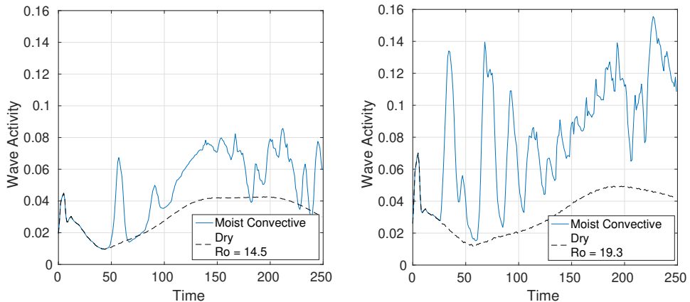
FIGURE 11. Wave activity measured as the modulus of divergence integrated over the region beyond the radius of maximum wind during the evolution of TC-like vortices with different Rossby numbers in dry and moist-convective environments. Ro = 14.5 (left panel, ID : Dbis3, MCbis3 ), Ro = 19.3 (right panel, ID : Dbis4, MCbis4 ), respectively.
