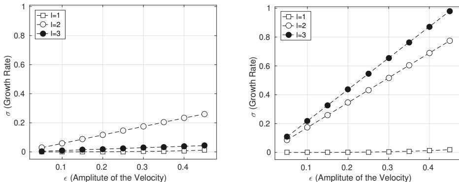
FIGURE 2. Growth rates of the azimuthal modes l = 1, 2, 3 as functions of the vortex intensity. Left and right panels correspond to the upper- and lower- row configurations presented in figure 1, respectively.
