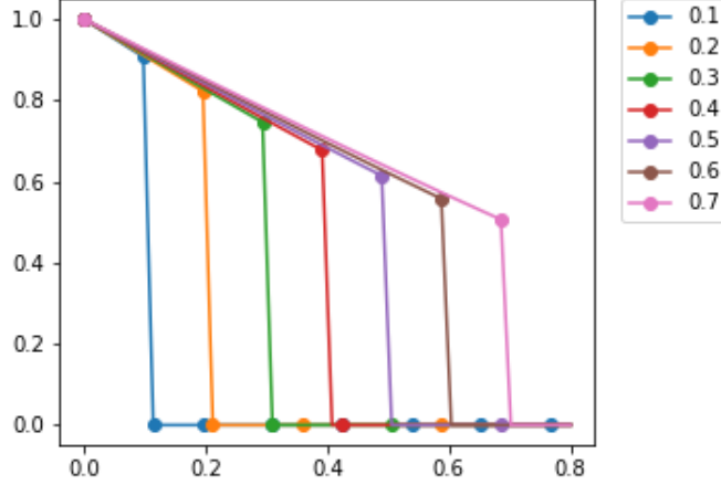
Figure 1: Solution X/\Delta X of the Stokes first problem given by (84) as a function of y = b/\lambda\sqrt{\mathcal{G}_\epsilon} at t/\lambda \in \{.1, .2 \dots .7\} using numerical integration.
