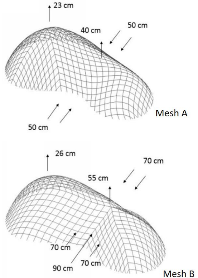
Figure 13. Meshes A and B after relaxation.
