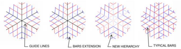
Figure 15. Procedure for extending the bars at edge-lines.
