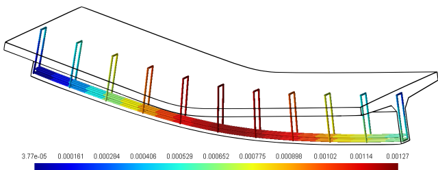
Fig. 9 3D viewing of the displacement of rebars (absolute displacement in meters)
