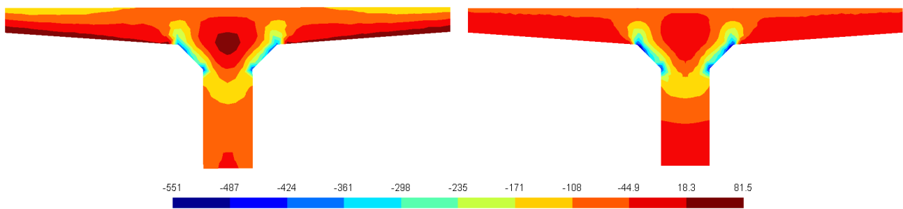
(b) \sigma_{22} computed from the beam solution (left) and from the reference solution (right) in kPa
