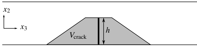
Fig. 23 Definition of the potential cracked area
