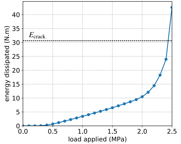
Fig. 24 Energy dissipated in V_{\text{crack}} as function of the load applied
