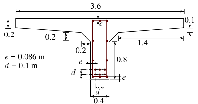
Fig. 3 Geometry of the T-beam section (dimensions in m)
