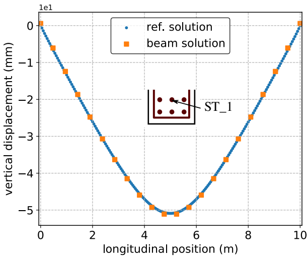
(b) Vertical displacement in rebar ST_1
