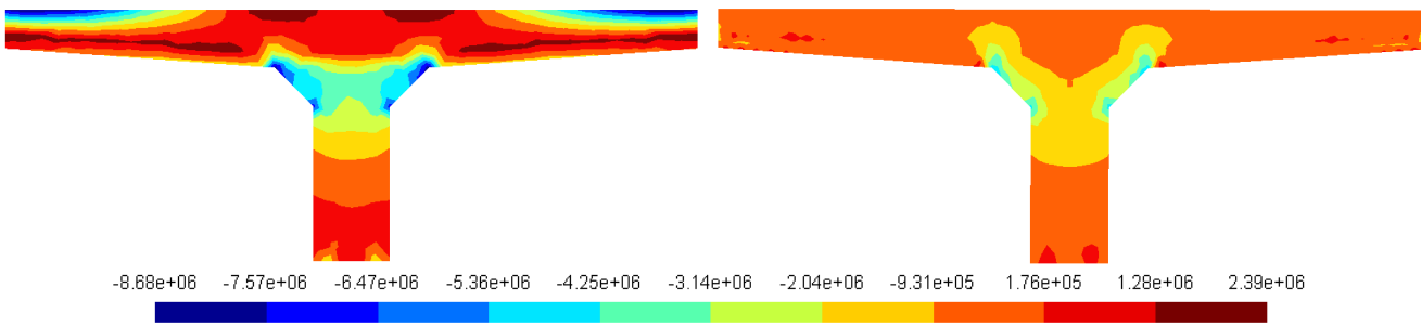
(b) \sigma_{22} computed from the beam solution (left) and from the reference solution (right)
