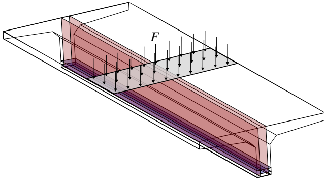
Fig. 4 Surfaces modeling rebars as membranes in the reference solution and description of the load
