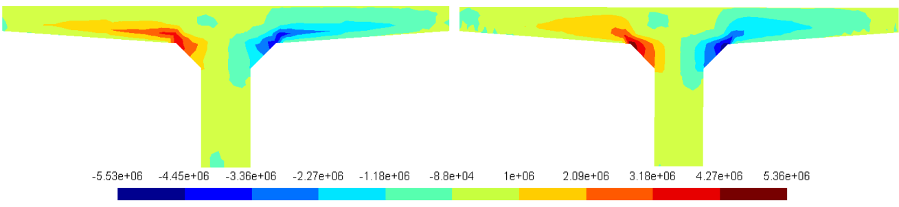
(d) \sigma_{12} computed from the beam solution (left) and from the reference solution (right)
