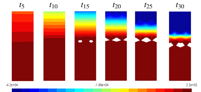
Fig. 22 Evolution of the normal stress \sigma_{33} (kPa) in the mid-span cross-section ( x_3 = 5 m)
