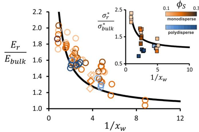
Figure 6: Evolution of the elastic stiffness of foam ribbons E_r as a function of the thickness-to-pore size ratio 1/x_w = e/\langle D_p \rangle . Presented data correspond to those of Fig. 4 (circles Fig. 4a, diamonds Fig. 4b). Solid fractions \phi_s is indicated by the color scales. The solid line corresponds to the following relation: E_r/E_{bulk} = 1 + 1.1 \langle D_p \rangle/e with E_{bulk} = 0.62\phi_s^{1.45} . Inset: Evolution of the rupture stress \sigma_r^* of foam ribbons as a function of the thickness-to-pore size ratio 1/x_w = e/\langle D_p \rangle . Solid fractions \phi_s is indicated by the color scales. The solid line corresponds to the following relation: \sigma_r^*/\sigma_{bulk}^* = 1 + 1.1 \langle D_p \rangle/e with \sigma_{bulk}^* = 3500\phi_s^{1.2} .
