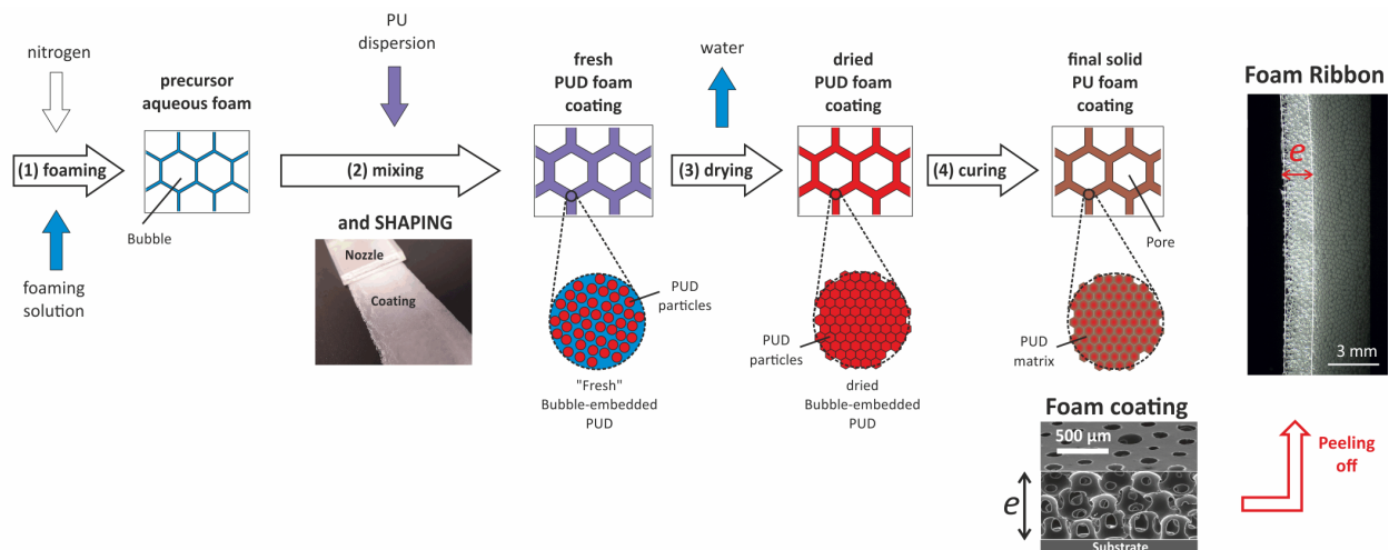
Figure 1: Sketch showing the main steps of the method used to produce solid polymer foams from aqueous polyurethane dispersion (PUD). (1) The precursor aqueous foam is made by using microfluidics. The bubble/pore size is set at this stage. (2) The precursor foam is mixed with the polyurethane dispersion. The PU content is set by volume flow rates of precursor foam and PUD. At this stage the shape of the ribbons is set by spreading the fresh PUD foam on a solid substrate. The thickness of the foam coating is set by the spreading velocity. (3) The fresh PUD foam is dried for 12h in a climatic chamber. (4) The dried PUD foam is cured at 150^\circ\text{C} for 15 min in order to activate the cross-linker. The resulting open-cell solid foam coating has pore size D_p equal
