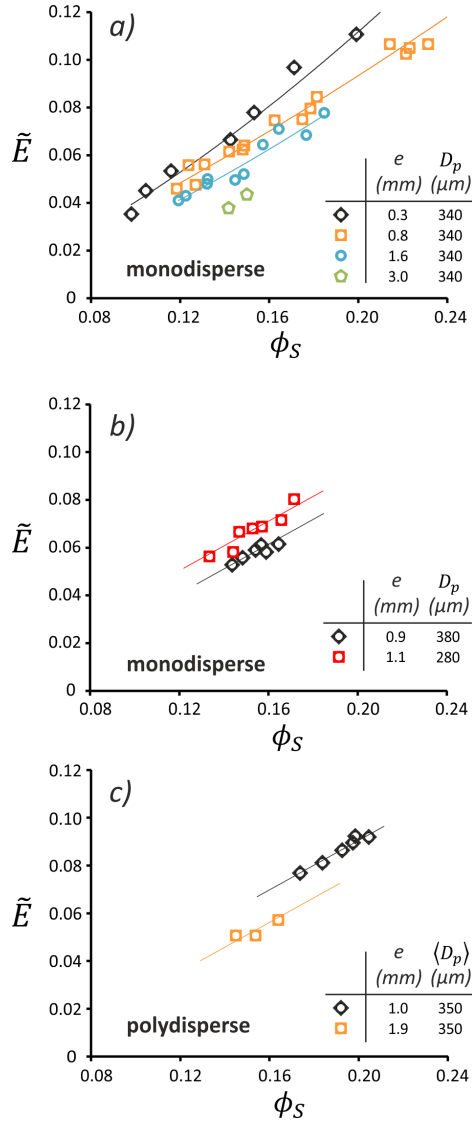
Figure 4: Dimensionless tensile stiffness measured for foam ribbons as a function of solid volume fraction, for different pore sizes D_p and ribbon thickness e (as indicated in the figures). (a) Monodisperse foam: Effect of ribbon thickness for a fixed pore size. Solid lines correspond to fitted power laws, i.e. \tilde{E} = \alpha\phi_S^b , with a = 1.08 and b = 1.46 for e = 0.3 \text{ mm} , a = 0.74 and b = 1.28 for e = 0.8 \text{ mm} , a = 0.86 and b = 1.48 for e = 1.6 \text{ mm} . (b) Monodisperse foam: Effect of pore size for a fixed ribbon thickness. Solid lines are guides for the eye. (c) Polydisperse foam: Effect of ribbon thickness.
