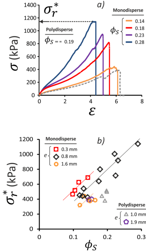
Figure 5: Large strain deformations of foam ribbons. (a) Typical stress-strain curves obtained for foam ribbons with thickness e = 810 \pm 40 \mu\text{m} . The pore size is D_p = 340 \mu\text{m} for monodisperse samples and \langle D_p \rangle = 350 \mu\text{m} for polydisperse samples. Note that rupture is observed for stress \sigma_r^* . (b) Rupture stress \sigma_r^* as a function of \phi_S for both monodisperse ( D_p = 340 \mu\text{m} ) and polydisperse ( \langle D_p \rangle = 350 \mu\text{m} ) foam ribbons with different thicknesses (as indicated). Solid straight lines are guides for the eye.
