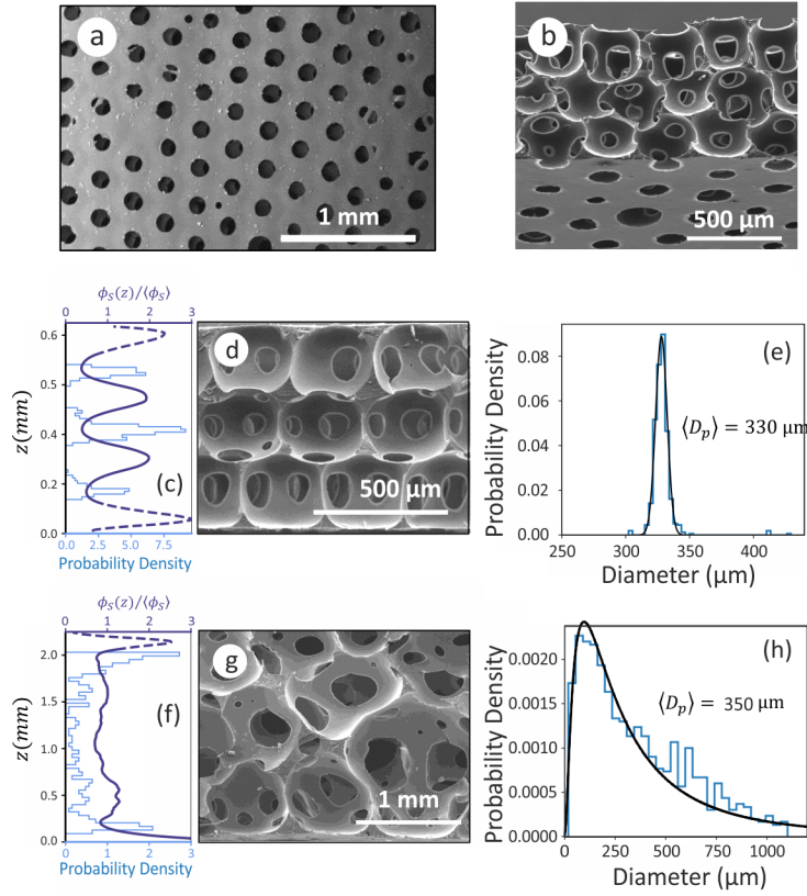
Figure 2: Typical examples of foam ribbon samples made in this study. (a) SEM picture showing the top free surface, where the pores of the top layer are open (monodisperse sample, pore diameter: 330\mu\text{m} ). (b) SEM picture showing the pore layer that was initially in contact with the substrate as well as the bulk pores (monodisperse sample, pore diameter: 330\mu\text{m} ). (c-e) monodisperse sample ( e = 830\mu\text{m} , \langle D_p \rangle = 330\mu\text{m} , \langle \phi_s \rangle = 0.14 ): (c) Typical solid volume fraction profile \phi_s(z) and pore position probability density measured across the ribbon's thickness e . Dashed curves indicate areas for which solid fraction should be considered as an "apparent" value due to the "roughness" at the free top surface of the samples. (d) SEM picture showing a side view of the sample. (e) number weighted pore diameter distribution. The solid line represents a normal distribution with parameters m_n=330 and \sigma_n=4.8 (respectively the mean and the standard deviation of the size distribution). (f-h) polydisperse sample ( e = 2250\mu\text{m} , \langle D_p \rangle = 350\mu\text{m} , \langle \phi_s \rangle = 0.13 ): (f) Typical solid volume fraction profile \phi_s(z) and pore position probability density measured across the ribbon's thickness e . (g) SEM picture showing a side view of the sample. (h) number weighted pore diameter distribution. The solid line represents a log-normal distribution with parameters m_{ln}=5.65 and \sigma_{ln}=1 (respectively the mean and the standard deviation of the size's natural logarithm).
