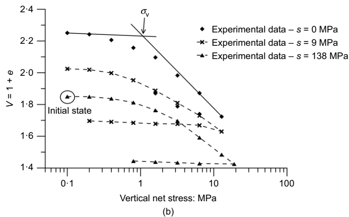
Fig. 17. (a) Experimental set-up for suction-controlled oedometer tests. (b) Results from suction-controlled oedometer tests on MX80 pellet/powder bentonite mixture (80/20) prepared at a dry density equal to 1.49 \text{ Mg/m}^3
