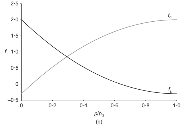
Fig. 12. Double-structure deformation model for expansive clays: (a) microstructural model; (b) interaction functions
