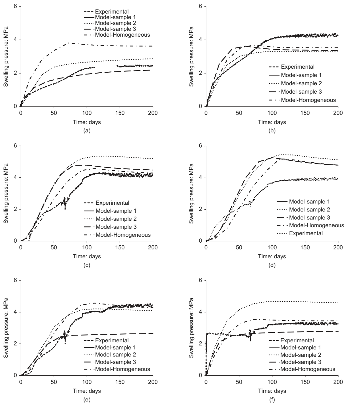
Fig. 22. Evolution of swelling pressure at different positions for the mock-up test together with model results of three different samples and a homogeneous case: (a) axial; (b) SP20; (c) SP40; (d) SP60; (e) SP80; (f) SP100
