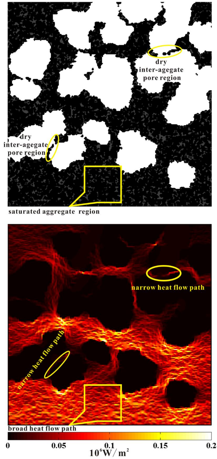
Fig. 11. Multi-phase distribution at the second water content ( e_w=e_m ) in the upper half and its corresponding heat flux density field in the lower half.
