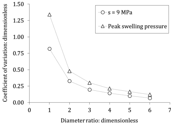
Fig. 9. Calculated coefficient of variation of the swelling pressure as a function of the ratio of pressure sensor diameter to initial pellet diameter.
