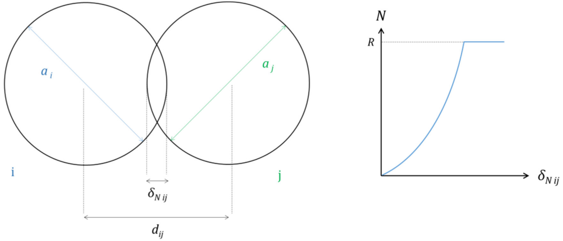
Fig. 4. Left: contact between two pellets i and j of diameter a_i and a_j , distance between centres d_{ij} , and normal deflection \delta_{N\,ij} . Right: evolution of normal force as a function of normal deflection.
