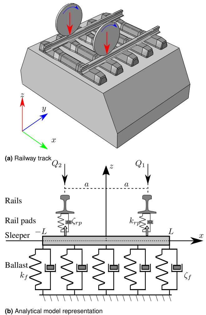
Figure 1. Railway track (a) and the analytical model representation (b)
