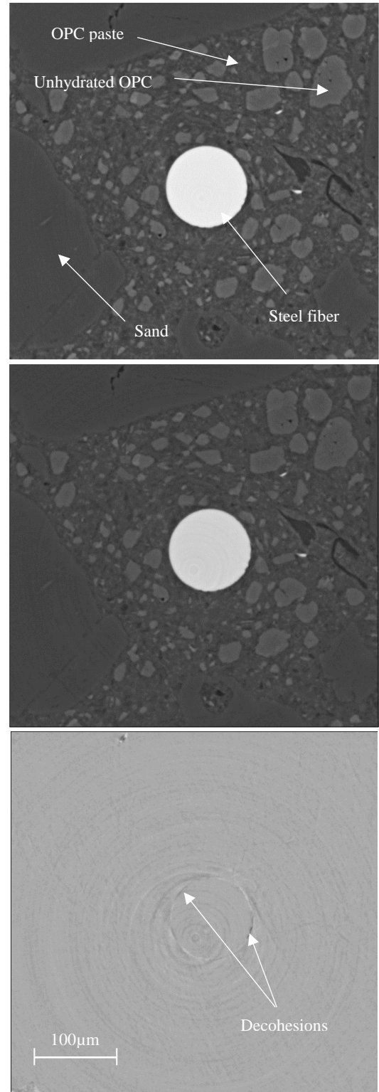
Figure 8: Zoomed cross-section of stainless steel reference subvolume (top), rebuilt damaged subvolume at 15N (top), subtracted subvolume (bottom)
