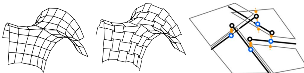
Figure 6: Initial PQ-mesh (left), structure obtained by translation of the edges: the opposite edges of the quads remain co-planar (middle), zoom on resulting eccentricities between members (right)
