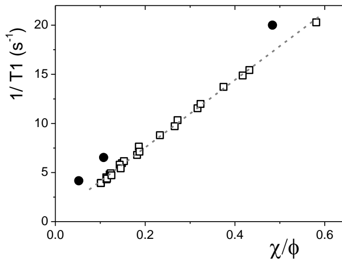
Figure 4 : NMR relaxation in silica particles suspensions. Measured 1/T_1 values as a function of particle to water volume ratio (squares). Similar measurements for suspensions as interstitial fluid in a saturated bead packing (circles). The grey line is the linear fit of equation (2) for suspensions with \alpha = 35.2 \text{ s}^{-1}
