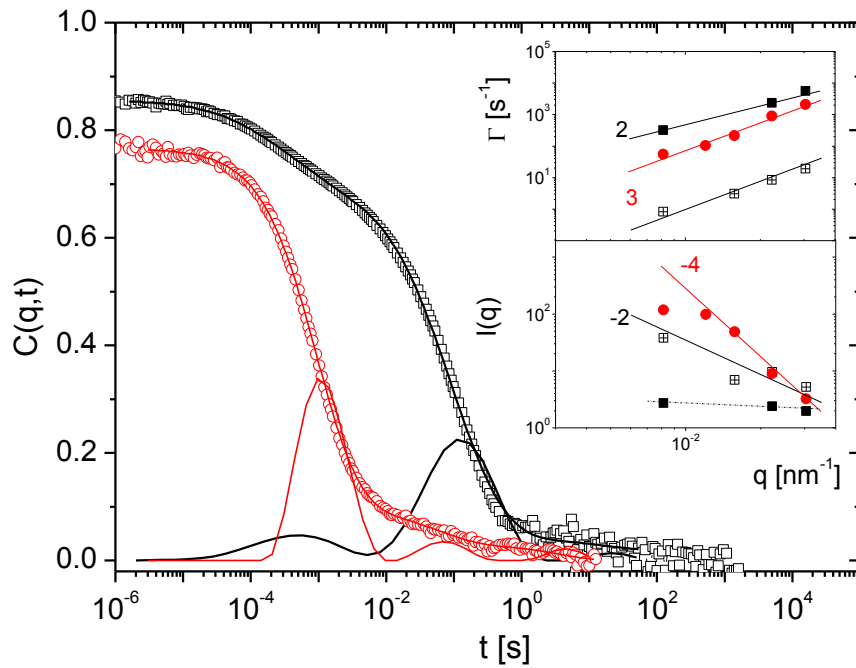
Figure 12: Normalized intermediate DLS function C(q,t) at q=0.022 \text{ nm}^{-1} and 20^\circ\text{C} , for the supernatant of the third centrifugation of the 0.34% wt aqueous CE solution (open squares, right). The respective C(q,t) after diluting this solution by 5000 times is also shown (open circles, left). The solid lines represent the distribution of relaxation times via CONTIN and the respective fits to C(q,t) . Insets: The dependence of the relaxation rates of the different modes of the correlation functions (top) and their (intensities) on q (see text). The lines are drawn to guide the eye and indicate the slopes (numbers).
