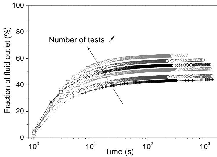
Figure 15: Fraction of fluid outlet, 1-WR , for successive filtration tests using only the solution outlet of the previous test for a 0.34 wt.% CE solution with a 100 \mu\text{m} sieve at a initial height of 20cm.
