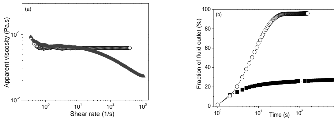
Figure 14: (a) Apparent viscosity of the oil (empty circles), and a 0.34% wt MH100000 CE solution (filled triangles). (b) Fraction of fluid outlet 1-WR for oil (circles) and a 0.34% wt CE solution (squares) through a sieve of 80 \mu\text{m} mesh width and for an initial height of 10 cm.
