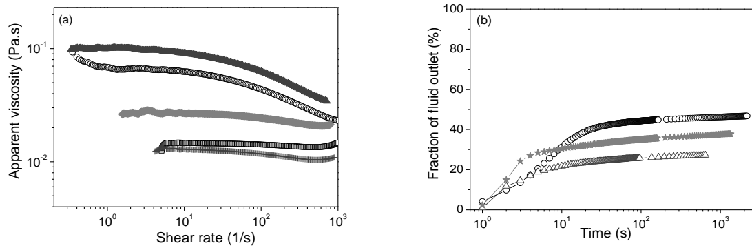
Figure 16: (a) Impact of surfactant on a 0.34% wt CE suspension apparent viscosity: without SDS (empty circles), with 10mmol/L SDS (filled triangles), 15mmol/L SDS (filled diamonds) and 20mmol/L SDS (empty squares); compared with a 0.17% wt CE suspension (plus sign). (b) Fraction of fluid outlet, 1-WR , for 0.17% wt (filled stars) and 0.34% wt MH100000 suspensions without (empty triangles) and with 15mmol/L SDS (empty circles) through a 80\mu\text{m} sieve and for an initial height of 10 cm.
