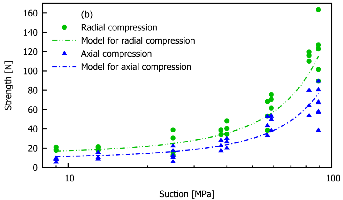
Figure 9: Strength versus modulus for both axial and radial compression tests.
