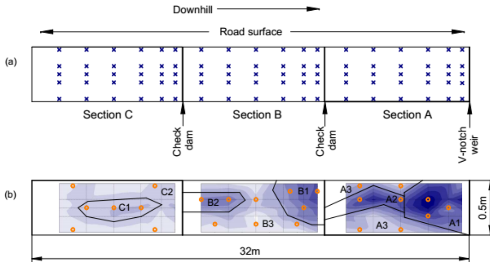
Figure 2. Schematic of (a) surface soil sampling and (b) core sampling of the biofiltration swale in Compans. Surface samples were taken at each blue x (a), while cores were taken at each orange circle and mixed according to zones (A1, A2, A3, B1, B2, B3 and C1, C2) selected based on the cartography of copper concentrations shown in the background (b). Please note that horizontal and vertical scales are different.
