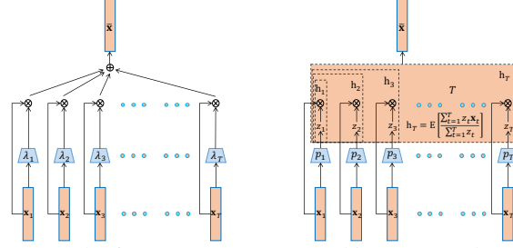
Figure 4: The feature aggregators used in STPN and MAAN.
