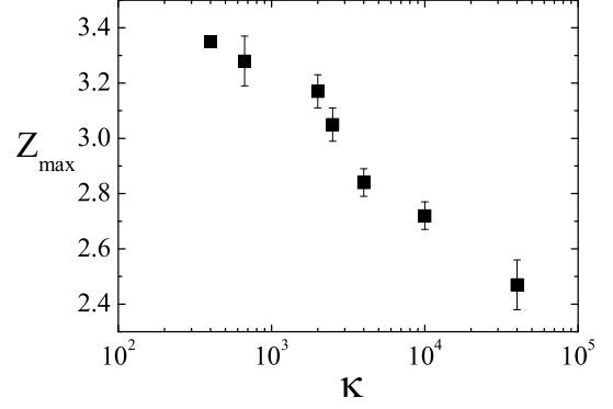
FIG. 12: Variation of the maximum coordination number as a function of \kappa ( e = 0.1 , \mu = 0.4 ).
