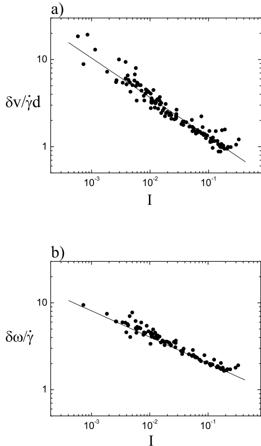
FIG. 10: Relative velocity fluctuations as a function of I : (a) Translation velocity, (b) Rotation velocity (various parameters).
