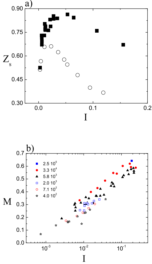
FIG. 13: (Color online) (a) Variation of Z_s as a function of I ( \mu = 0.4 - \kappa = 4000 - e = 0.1 (■), e = 0.9 (○)) (b) Variation of M as a function of I , for various \kappa .
