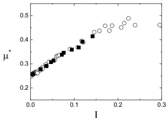
FIG. 3: Friction law ( \mu = 0.4 , e = 0.1 (o), e = 0.9 (■), various \kappa ).
