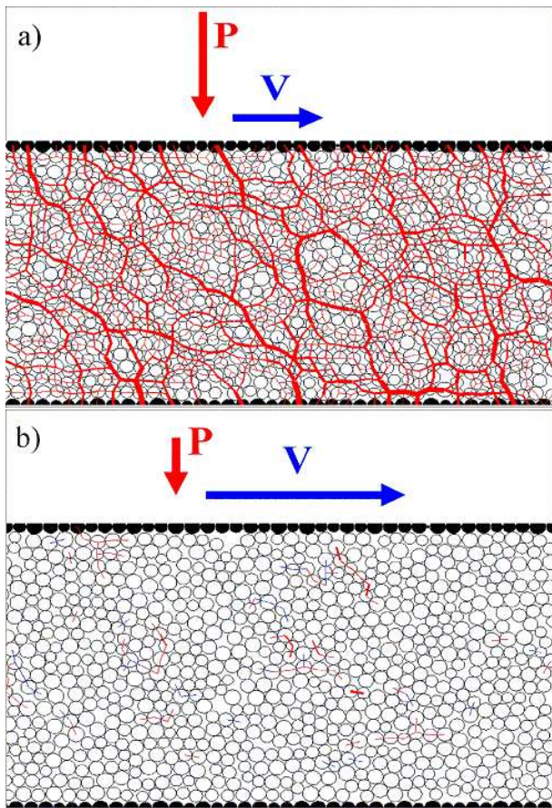
FIG. 1: (Color online) Plane shear : (a) Quasi-static regime ( I = 10^{-2} ) (b) Collisional regime ( I = 0.2 ). (Black grains constitute the rough walls. The line widths are proportional to the intensity of the normal force between grains).
