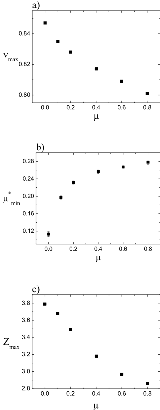
FIG. 5: Influence of \mu on the critical state ( I = 4 \cdot 10^{-3} and e = 0.1 ): (a) Maximum packing fraction \nu_{max} , (b) Effective friction coefficient \mu_{min}^* , (c) Coordination number Z_{max} .
