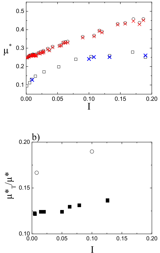
FIG. 16: (Color online) Friction and anisotropy : (a) Comparison of Eqn. 34 (cross) with direct measurement of Fig. 6 (open symbols) ( \mu = 0 ( \square ), \mu = 0.4 ( \circ )), (b) Tangential contribution for \mu = 0.4 ( \blacksquare ) and \mu = 0.8 ( \circ ).
