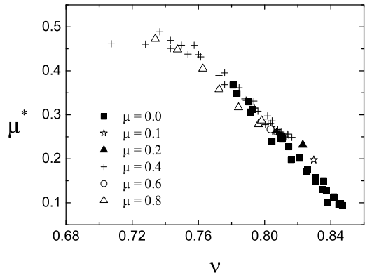
FIG. 7: Variation of the effective friction coefficient as a function of solid fraction.
