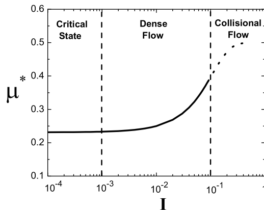
FIG. 17: Diagram of the granular flow regimes.
