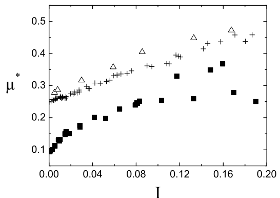
FIG. 6: Influence of \mu on the friction law ( \mu = 0 (■), \mu = 0.4 (+), \mu = 0.8 (△), various e ).
