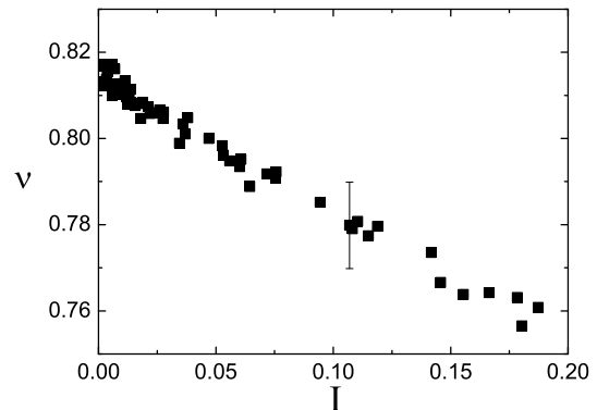
FIG. 2: Dilatancy law ( \mu = 0.4 , various e and \kappa ).
