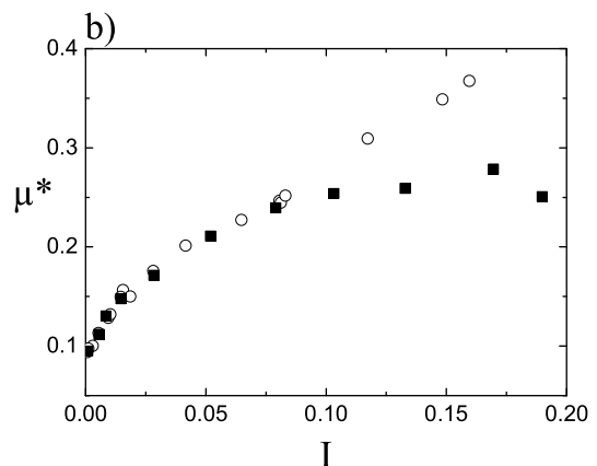
FIG. 8: Influence of e for \mu = 0 ( e = 0.9 (■), e = 0.1 (○)) : (a) Dilatancy law, (b) Friction law.
