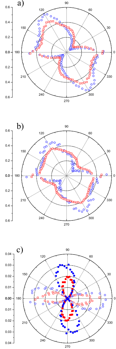
FIG. 14: (Color online) Angular distribution of the contact forces (quasi-static regime ( I = 0.005 - □), collisional regime ( I = 0.13 - ○): (a) \zeta_N(\phi) ( \mu = 0.4 ), (b) \zeta_N(\phi) ( \mu = 0 ), (c) \zeta_T(\phi) ( \mu = 0.4 ) - \geq 0 white symbols, \leq 0 black symbols.
