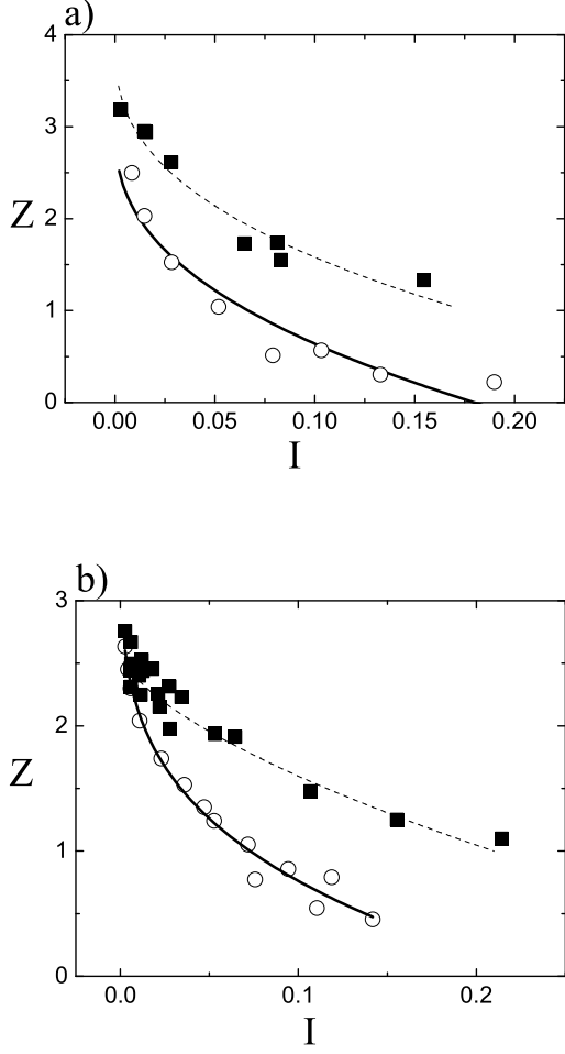
FIG. 11: Variation of the coordination number Z as a function of I ( \kappa = 10^4 , e = 0.1 ( \blacksquare ), e = 0.9 ( \circ )) (a) \mu = 0 - Fits Z = 3.75 - 7.11I^{0.51} (---), Z = 3.00 - 6.04I^{0.41} (-) (b) \mu = 0.4 - Fits Z = 2.84 - 3.80I^{0.48} (---), Z = 2.60 - 5.48I^{0.50} (-).
