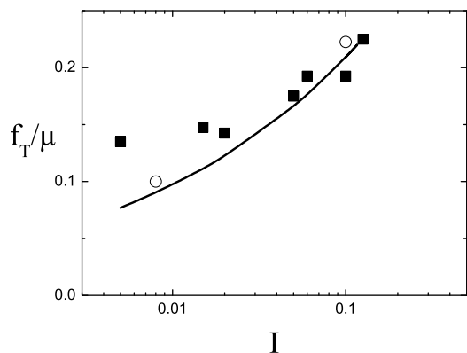
FIG. 15: Angular distribution of tangential contact forces: (a) \zeta_T(\phi)/\zeta_N(\phi) ( \circ ) fitted by f_T \cos(2\phi) (—) for I = 0.13 and \mu = 0.4 , (b) f_T(I)/\mu for \mu = 0.4 ( \blacksquare ) and \mu = 0.8 ( \circ ) compared with \frac{\sqrt{2}}{\pi} I^{1/3} .
