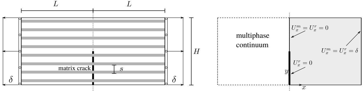
Figure 10: Left: Tension of a multilayered medium with a matrix crack bridged by reinforcements. Right: Boundary conditions for the associated multiphase model.
