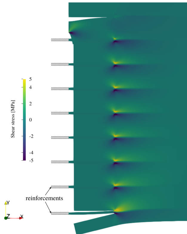
Figure 14: Close-up on the shear stress field near the delaminated zone (heterogeneous FE computations)
