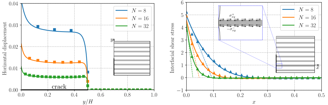
(a) Matrix displacement (averaged over each matrix layer for the heterogeneous model)
