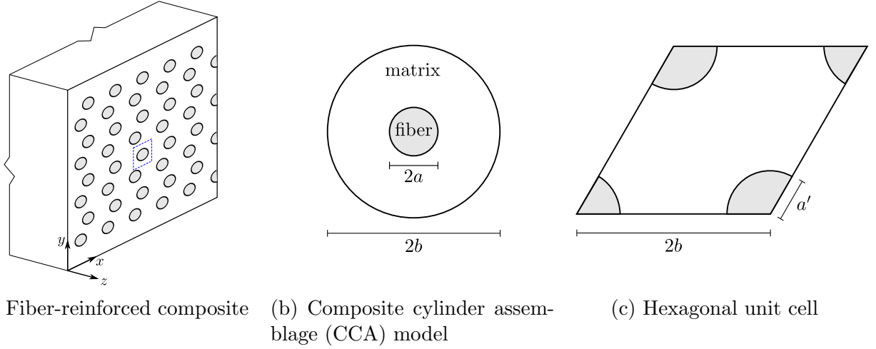
Figure 4: Unidirectional fiber-reinforced composite and associated microstructure models
