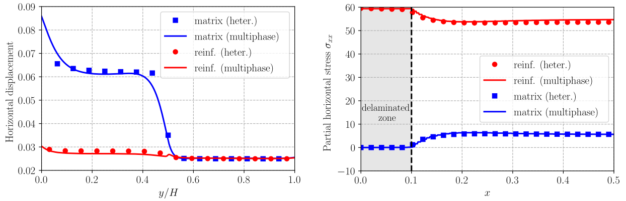
(a) Displacements along a vertical line at x = 0.05 (halfway through the delaminated zone)
