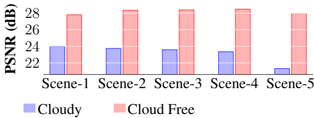
Fig. 5: Quantitative results on Synthetic Scenes
