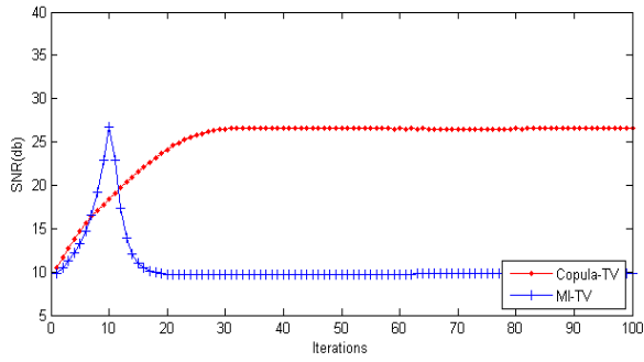
Figure 15: Average output SNRs versus iteration number: Uniform dependent sources from Clayton-copula.
