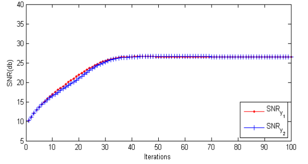
Figure 8: Average output SNRs versus iteration number : Bpsk dependent sources from Clayton-copula.
