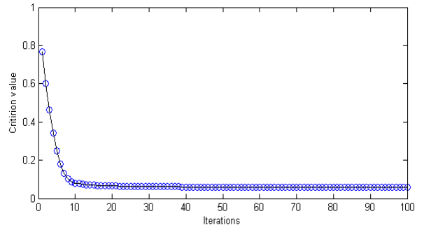
Figure 10: The criterion value vs iterations : Uniform dependent sources from FGM-copula.
