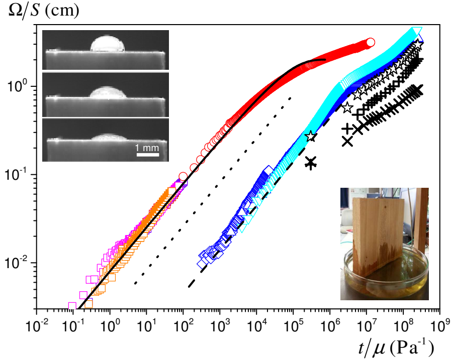
Figure 6 : Imbibition tests in longitudinal direction of poplar. Absorbed liquid volume per unit transversal cross-section area as a function of time (scaled by the liquid viscosity) from standard imbibition (20 mPa.s silicon oil : \circ , water: \triangle , water+betaine: \nabla ) or droplet imbibition tests (water: \diamond , silicone oils of viscosity 20 mPa.s, 125 mPa.s, 350 mPa.s, 500 mPa.s :all shown in \square ). The star symbols correspond to water amount as deduced from MRI (see Figure 9): bound water ( \times ), free water ( + ), total water amount ( \star ). The dotted line of slope \frac{1}{2} is a guide for the eye. The solid line is a possible fit of the Washburn equation taking into account gravity (equation (7)). The dash line corresponds to the diffusion model (see text) with D = 5.8 \times 10^{-9} \text{ m}^2 \cdot \text{s}^{-1} . The left top inset shows successive steps of droplet imbibition. The right bottom inset shows an image of the principle of imbibition setup from a bath (here without paint and bath cover for demonstration).
