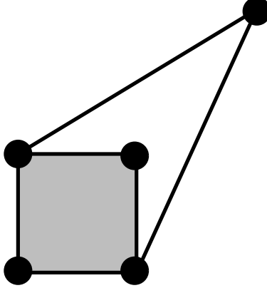
FIGURE 1. A 2-dimensional geometric cubical complex which is not the geometric realization of an abstract simplotopal complex as defined in the present paper
