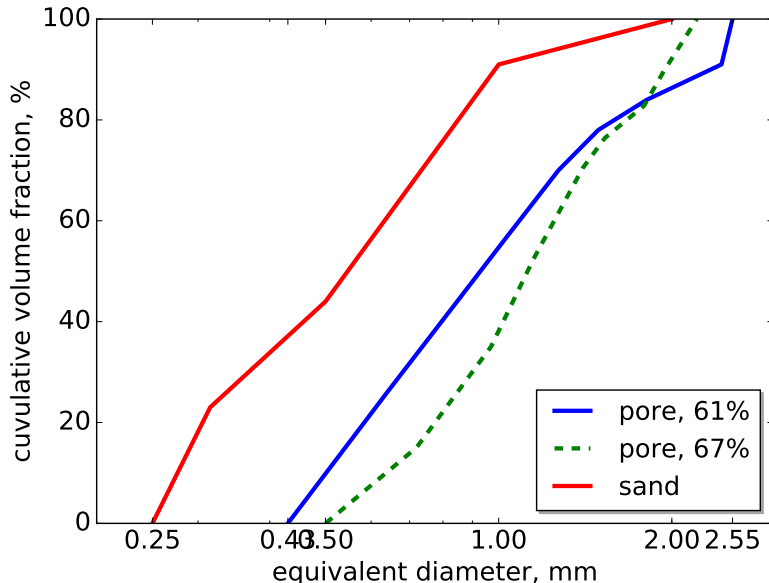
Figure 1.2: Pore size distributions are extracted from tomographic images at the Navier Laboratory and the size distribution of sand grains is obtained by using sieves. The pore size distribution slightly depends on the amount of foam added to the mix, i. e. the porosity.
