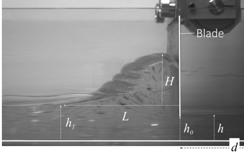
Figure 6: Notations. The picture here corresponds to the flow of the fluid with a yield stress \tau_c = 49 Pa, at a blade velocity V = 50 mm/s, an initial layer thickness h_1 = 10 mm and a gap h_0 = 5 mm.
