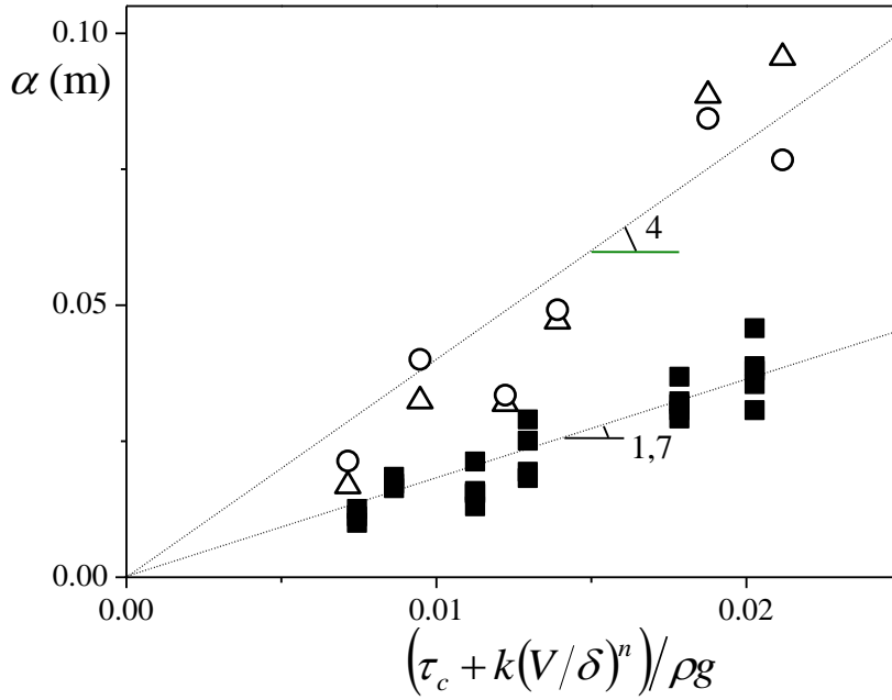
Figure 13: Values of \alpha as a function of the shear stress scaled by gravity for all the tests: (filled squares) our different data for h_0 \geq 7 mm ; (triangles) h_0 = 2 mm and h_1 = 7 mm , (circles) h_0 = 2 mm and h_1 = 5 mm .
