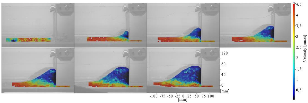
Figure 12: Evolution of the experimental horizontal velocity field during the blade-coating in a channel filled with yield stress fluid ( \tau_c = 98 Pa, V = 5 mm/s, h_1 = 17 mm, h_0 = 7 mm). The pictures correspond to successive steps of displacement of 100 mm. In this representation the blade has a velocity equal to zero (dark blue) while the channel has a velocity V (red). The color bar is in mm/s.
