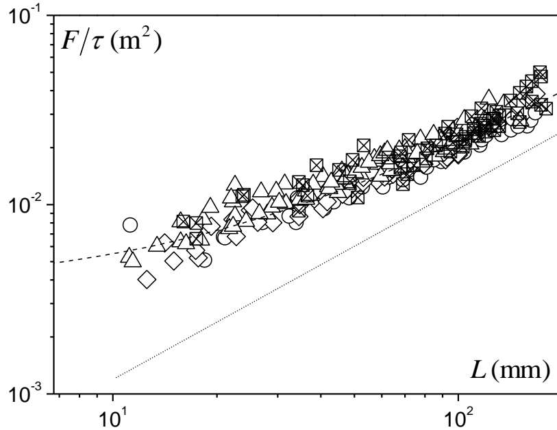
Figure 14: Force scaled by the shear stress (see text) as a function of the length of the shear-band for all our tests (see Table 1) at velocity V = 50 \text{ mms}^{-1} : \tau_c = 42 \text{ Pa} (circles), \tau_c = 49 \text{ Pa} (diamonds), \tau_c = 98 \text{ Pa} (triangles). Data corresponding to a velocity V = 1 \text{ mms}^{-1} and \tau_c = 98 \text{ Pa} are represented by crossed squares. The dotted line is equation (8) with \theta = 0 , the dashed line is equation (9).
