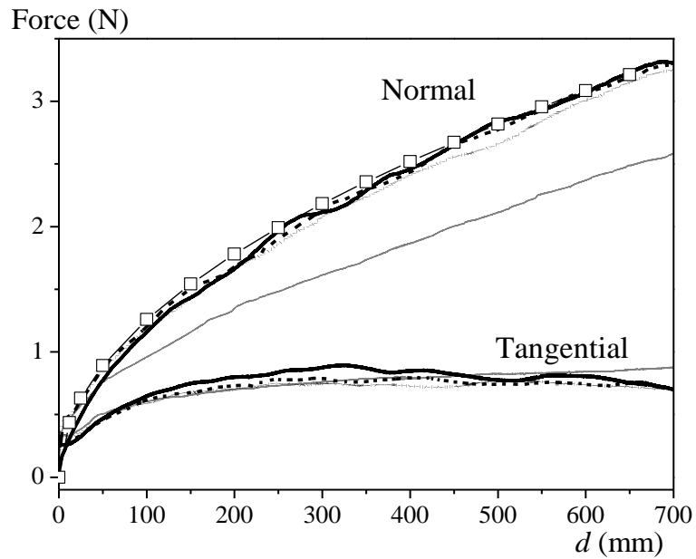
Figure 10: Tangential and normal forces as a function of the displacement for V = 5 mm/s, \tau_c = 98 Pa and: (thick continuous line) h_1 = 25 mm, h_0 = 20 mm, (thick dash line) h_1 = 20 mm, h_0 = 15 mm, (thick dotted line) h_1 = 15 mm, h_0 = 10 mm, (thin line) h_1 = 7 mm, h_0 = 2 mm. The symbols correspond to equation (3) with \beta = 0.126 \text{N} \cdot \text{mm}^{-1/2} .
