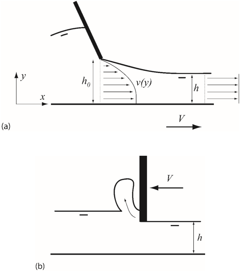
Figure 1: Schemes of the principle of blade-coating for fluids (a) and scratch test for solids (b).
