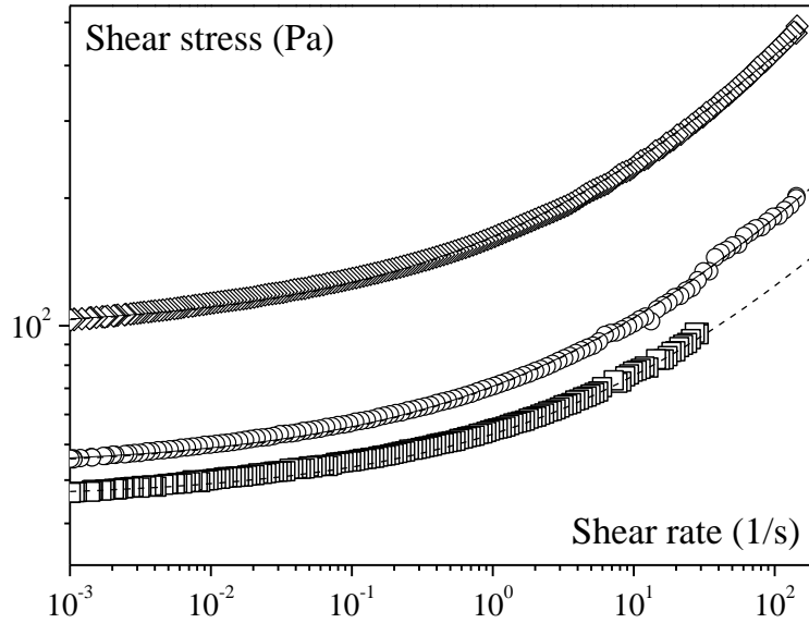
Figure 2: Flow curves of our Carbopol gels. The dashed lines correspond to a Herschel-Bulkley model fitted to data with n=0.35 and: \tau_c = 42 Pa, k = 16 Pa.s ^n (squares); \tau_c = 49 Pa, k = 24.5 Pa.s ^n (circles) and \tau_c = 98 Pa, k = 58 Pa.s ^n (diamond).
