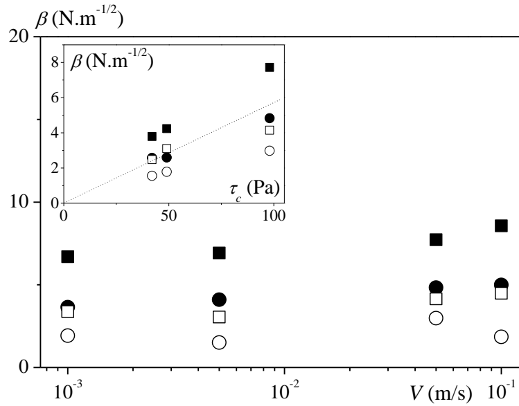
Figure 11: Values of the coefficient \beta (equation (3)) as a function of the blade velocity for \tau_c=98 Pa and: h_0 > 7 mm h_1 - h_0 = 10 mm (filled squares) or h_1 - h_0 = 5 mm (filled circles); h_0 < 7 mm and h_1 - h_0 = 5 mm (open squares) or h_1 - h_0 = 3 mm (open circles). The inset shows the variations of \beta as a function of the yield stress for V = 50 mm/s.
