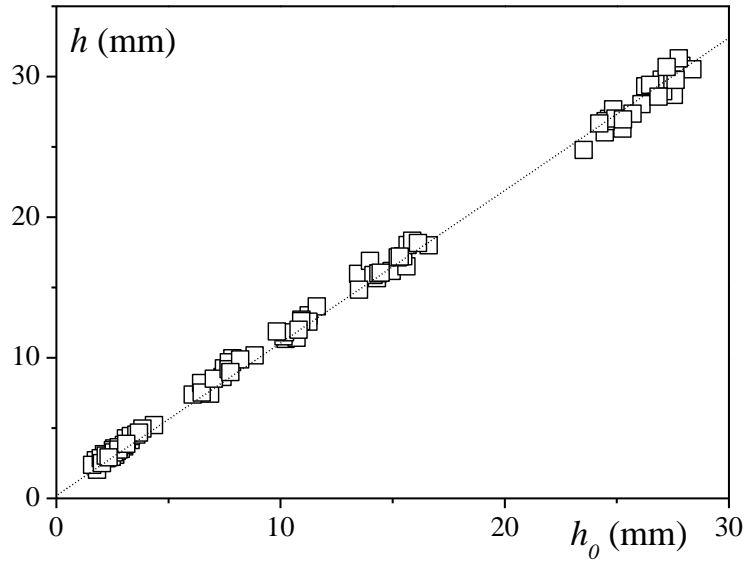
Figure 5: – Uniform coated layer thicknesses as a function of the gap between the blade and the plane for all the tests. The dotted line corresponds to equation (1).
