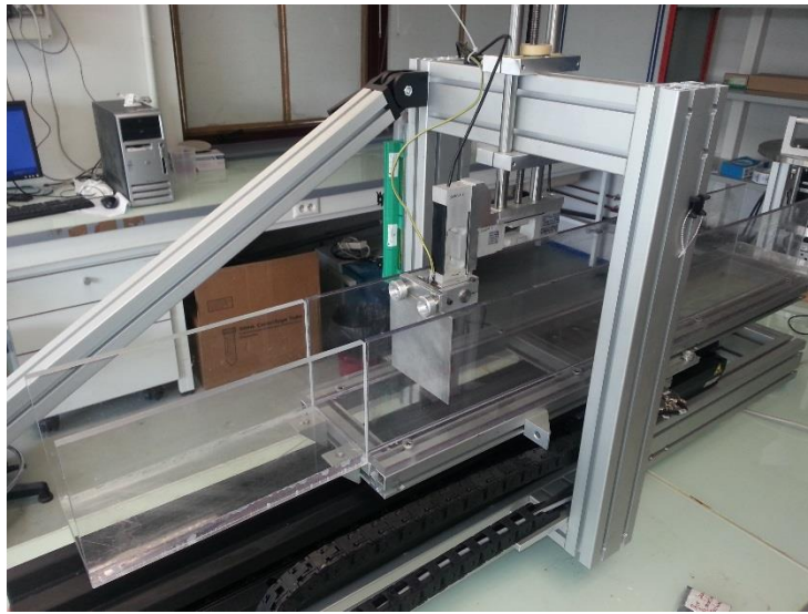
Figure 3: Overall view of the set up (camera not shown).
