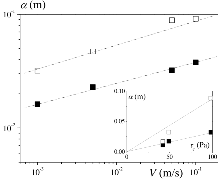
Figure 9: Values of the coefficient \alpha (equation (2)) as a function of the blade velocity for \tau_c=98 Pa and: (filled squares) h_1 = 20 mm , h_0 = 15 mm and (open squares) h_1 = 7 mm , h_0 = 2 mm . The inset shows the variations of \alpha as a function of the yield stress for V = 50 mm/s in these two situations.
