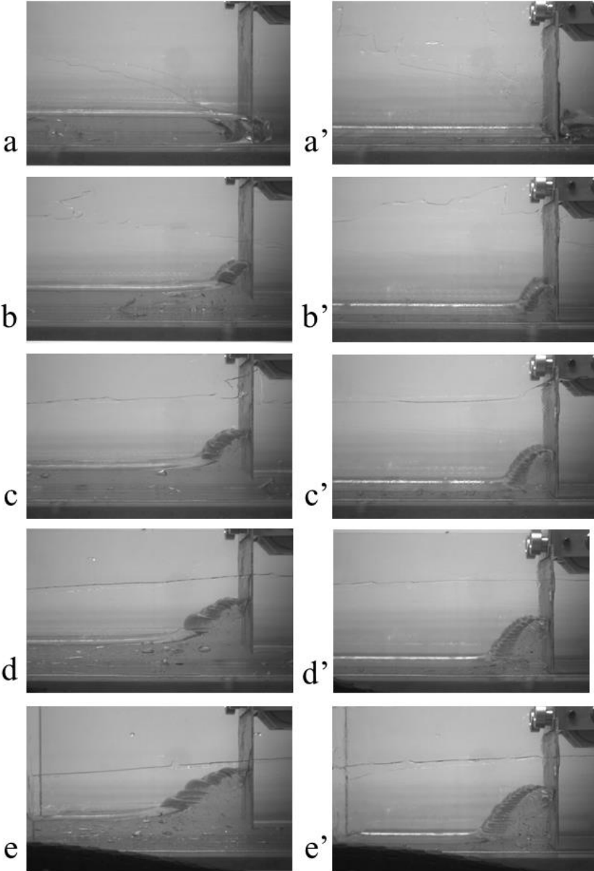
Figure 4: Aspect of the fluid at different times during the blade displacement (at a velocity V = 5\text{mm/s} ) over an initially uniform layer of yield stress fluid ( \tau_c = 98\text{ Pa} ): (left)
