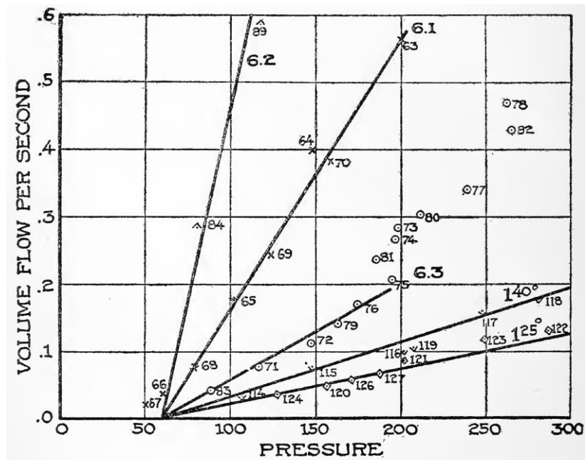
Figure 1: Key figure of Bingham's paper: Flow rate ( \text{mL}\cdot\text{s}^{-1} ) as a function of the pressure (in \text{g}\cdot\text{cm}^{-2} ) for a clay suspension flowing in capillaries of different diameters. The small numbers correspond to the test number, and the large number to the capillary diameter (see Bingham's paper for details).
