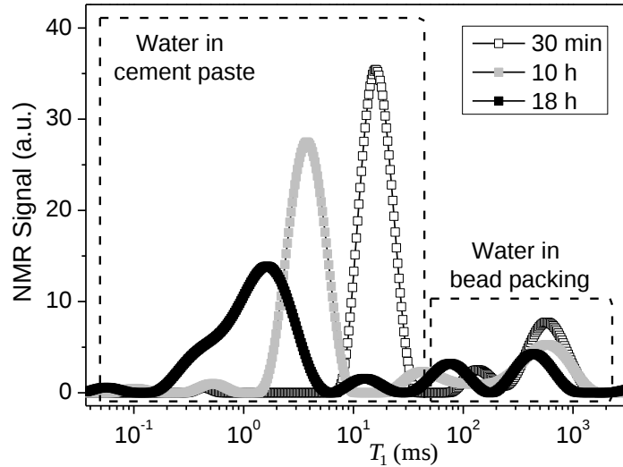
Figure 6. Distribution of relaxation time for a cement paste (initial W/C=0.4) in contact with a bead packing (A) at different times after the first contact. The dashed lines show the region of integration of the signal for estimating the water amount in each phase for the first distribution (i.e. 30 min).
