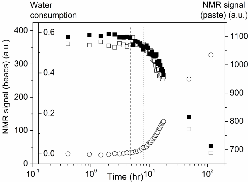
Figure 7. Evolution of water amount in the bead packing (empty squares) and in the paste (filled squares) as a function of time elapsed since the first contact between a cement paste (W/C = 0.5) and a bead packing (A). The water consumption (see text) is represented by circles. The dashed line marks the beginning of water consumption and the dotted line the beginning of water extraction from the bead packing.
