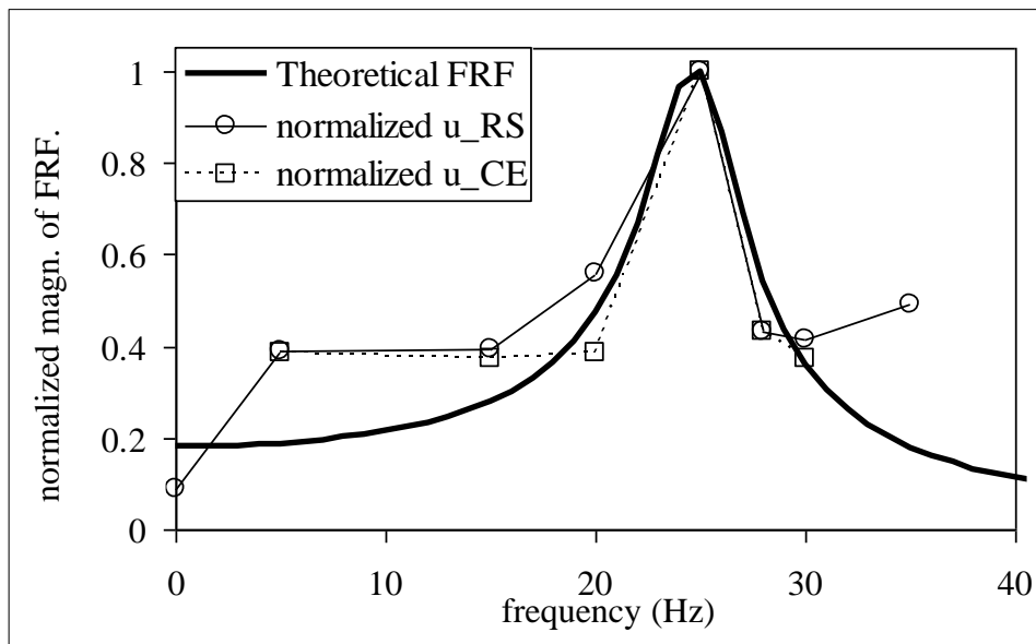
Figure 14 : Theoretical frequency response function vs. experimental mean horizontal facing displacements
