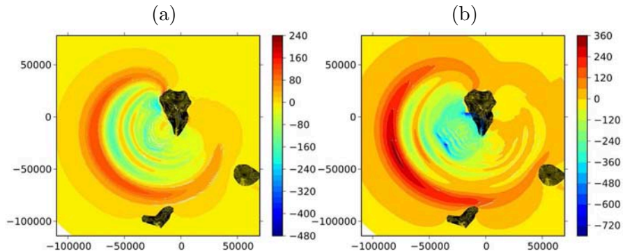
Figure 3. Surface elevations (color scale in meter) computed with THETIS for CVV flank collapse scenarios with volume: (a) 80 \text{ km}^3 , (b) 450 \text{ km}^3 , at t = 7.5 \text{ min} after the start of the event. Note, x and y axes represent distance in meter.
