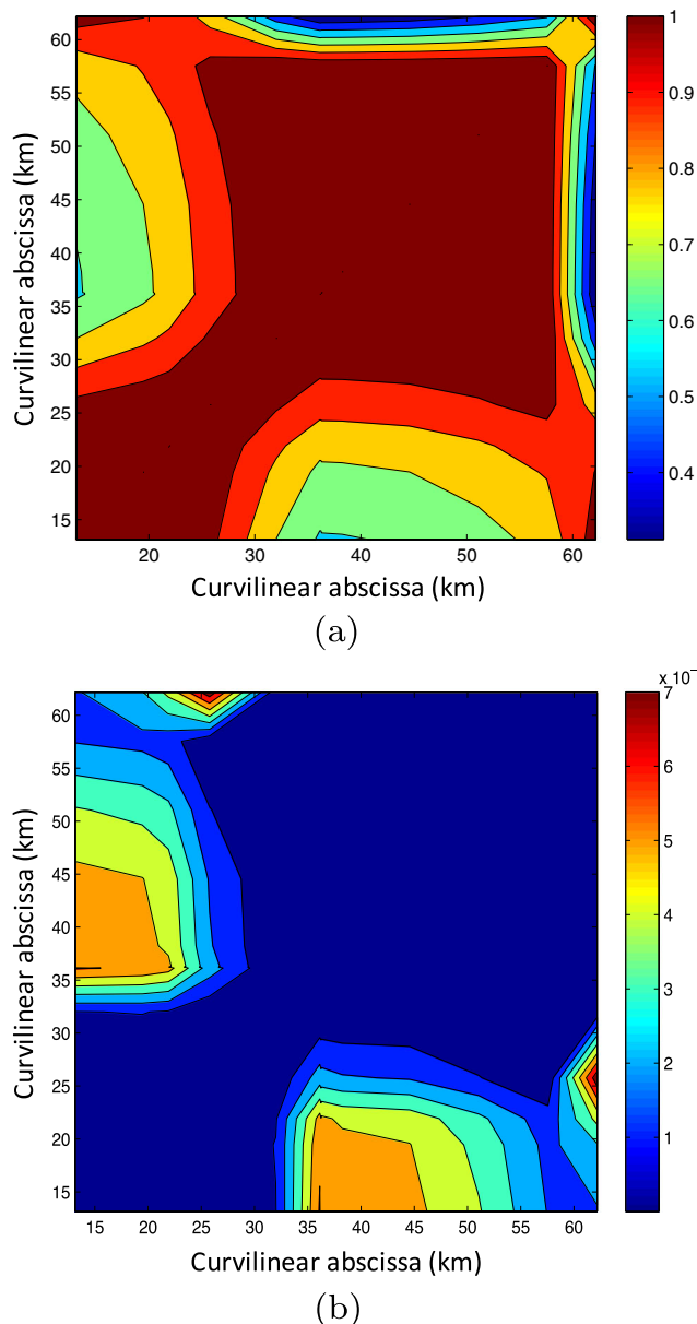
Fig. 16 Garonne River case in steady flow. a Water level correlation matrix over the 60-km Garonne reach estimated with the retained surrogate \mathcal{M}_{PC}^{quad7, P6} ( P = 6, n = 2 with \mathbf{x} = [Q, K_{s_3}]^T ). The colorbar represents the correlation in the water level error for each pair of grid points along the reach. b Error on the water level correlation matrix estimated \mathcal{M}_{PC}^{quad7, P6} with respect to the correlation computed with a MC sampling E_{MC} over N_{MC} = 10^5
