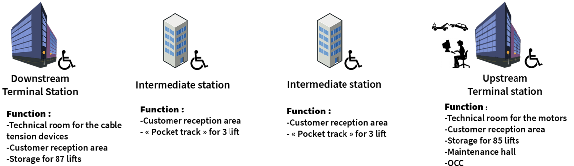
Diagram 3: Overall equipment diagram
