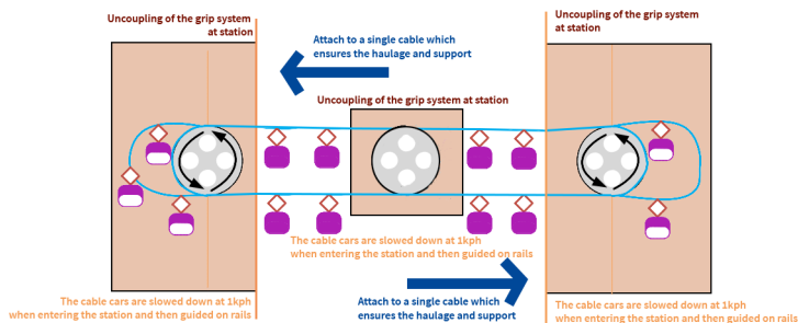
Diagram 2: Gondola lift system with single rope and a detachable grip
