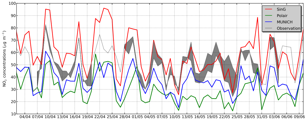
Figure 7. Temporal evolution of \text{NO}_2 daily-averaged concentrations modeled with MUNICH (blue line), Polair3D (green line), and the SinG model (red line). They are compared to the measured concentrations (gray shaded regions) at the stations nearby traffic on each sidewalk of the Boulevard Alsace-Lorraine. If the measurement is available at only one station, a black line is used instead.
