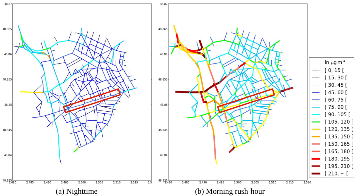
Figure 6. Simulated \text{NO}_x concentrations using MUNICH (a) during nighttime at 01:00 UTC and (b) in the morning rush hour at 07:00 UTC on 25 March 2014. The red rectangular box encompasses Boulevard Alsace-Lorraine and the cross mark corresponds to the location of the air monitoring stations on the sidewalks.
