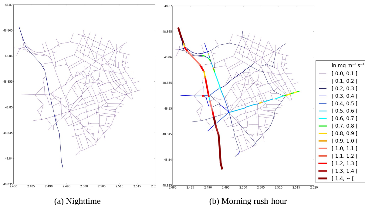
Figure 5. \text{NO}_x emission rates ( \text{mg m}^{-1} \text{s}^{-1} ) used in MUNICH simulations for a weekday (a) during nighttime at 01:00 UTC and (b) in the morning rush hour at 07:00 UTC on 25 March 2014.
