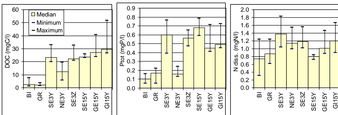
Figure 3 : range of dissolved organic carbon, total phosphorus and total dissolved nitrogen concentrations measured for runoff samples from the conventional flat roofs (BI: bituminous roof, GR: gravel roof) and from the 6 different vegetated roofs (SE3Y to GI15Y)
