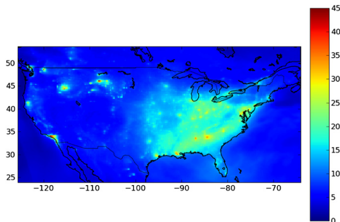
Fig. 5. Surface PM_{2.5} concentrations (in \mu\text{g m}^{-3} ) over North America averaged over July and August.
