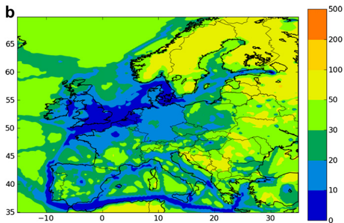
Fig. 7. Ratio of surface VOC over NO_x concentrations averaged over July and August computed using Pol 3 (Simpson biogenic emission scheme, upper panel) and Pol 4 (MEGAN biogenic emission scheme, lower panel).
