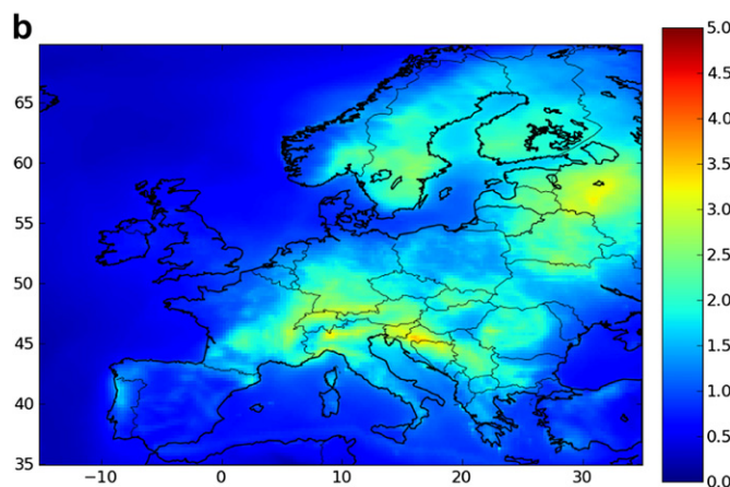
Fig. 3. Surface SOA concentrations (in µg m -3 ) over Europe averaged over July and August using Simpson (Pol 3, upper panel) and MEGAN (Pol 4, lower panel) biogenic emission schemes.
