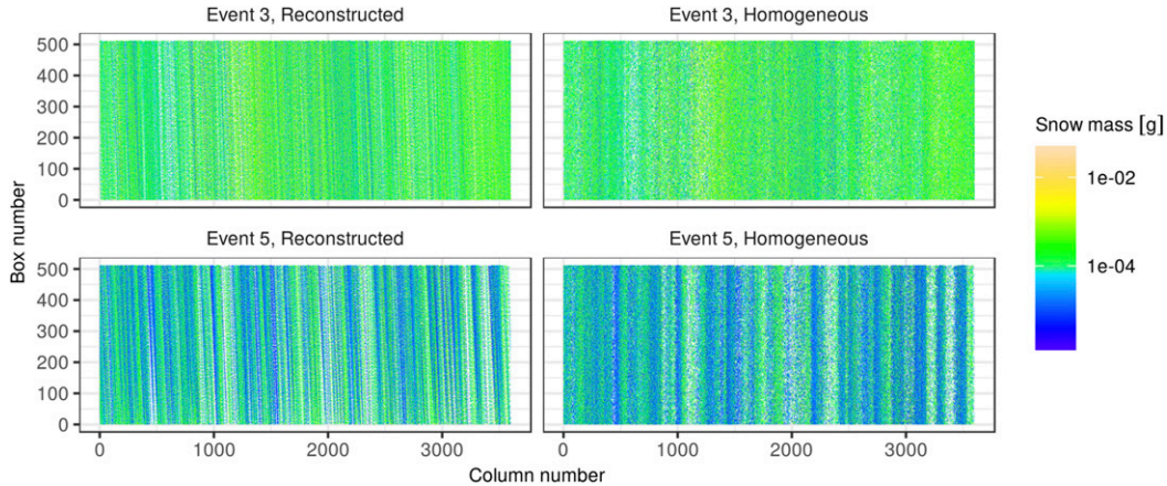
FIG. 4. Snow mass per box and per column, for events 3 and 5, showing the difference between reconstructed and homogeneously distributed particles. In the reconstructed fields, the particles falling toward the 2DVD over time are visible as oblique patterns. In the analyzed fields, zeros were filled in where no mass was recorded.
