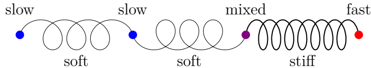
Figure 7: Example of system of particles with a slow-fast splitting
