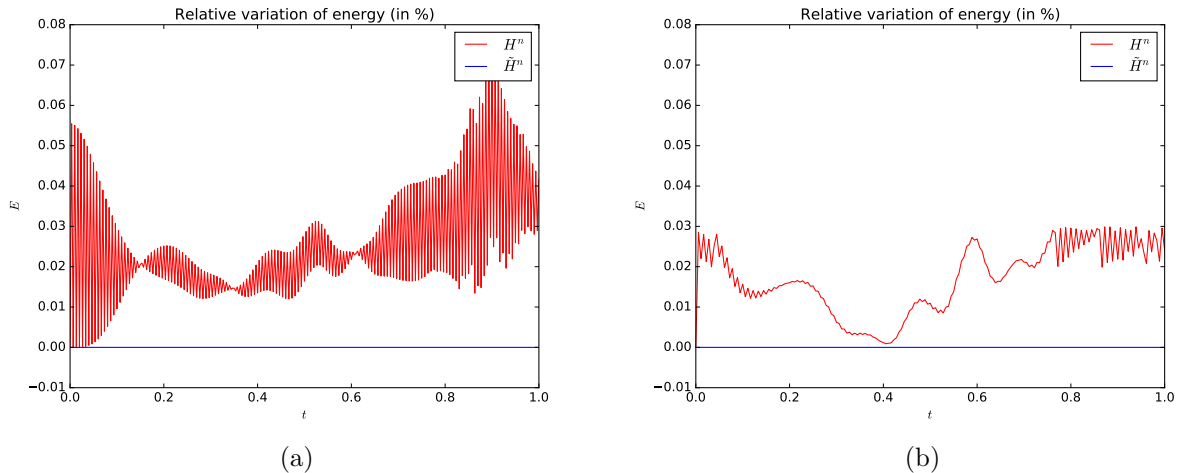
Figure 5: Nonlinear wave equation: time-variation of the discrete energy H^n and pseudo-energy \tilde{H}^n over a unit time interval for \alpha = 0.99 and an amplitude of 0.3 for u^0 : (a) Fixed time-step \Delta t = 0.0033 ; (b) Adaptive time-step as in Remark 8
