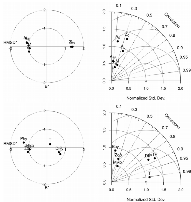
Figure 8: Target-Taylor diagrams for 0-20 m average concentration of (top) individual plankton groups and (bottom) dissolved phosphorus and total phosphorus, total phytoplankton, total mixotrophs and total zooplankton carbon biomass.
