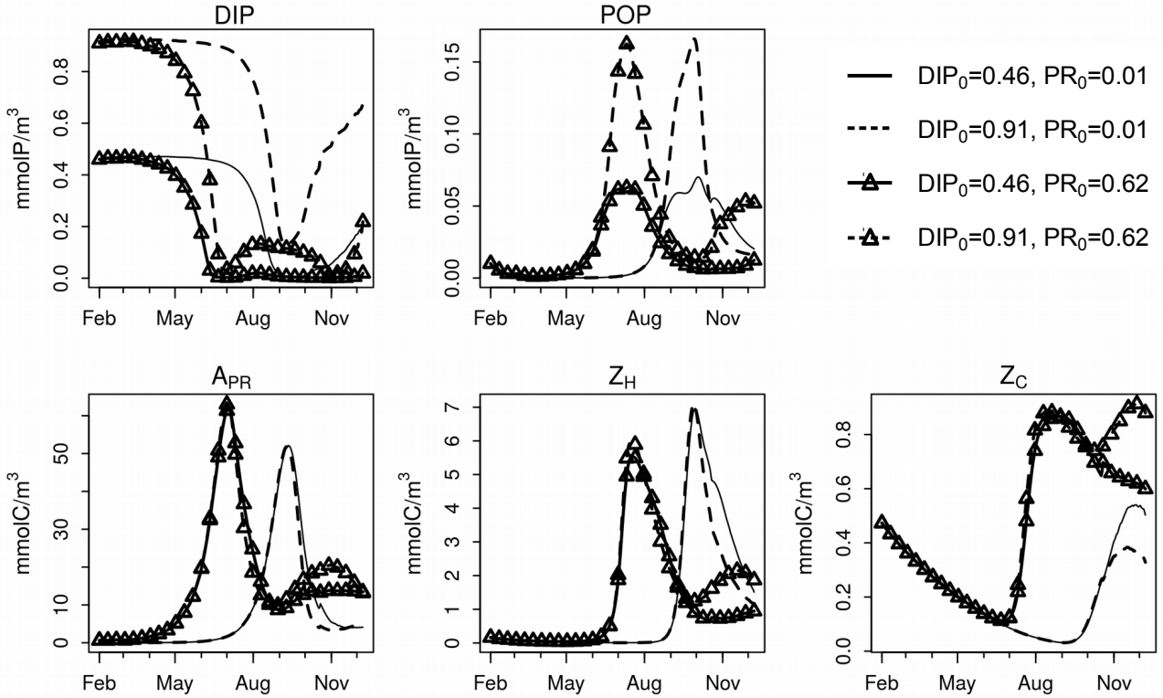
Figure B1: Surface (0-20 m) average water column average state variables with initial DIP concentration of DIP_0 = 0.46 \text{ mmolP m}^{-3} as in 2010 (solid lines), DIP_0 = 0.91 \text{ mmolP m}^{-3} as in 2004 (dashed lines), in combination with initial P. rubescens concentration of PR_0 = 0.01 \text{ mmolC m}^{-3} as (was assumed) in 2010 (no marker) and PR_0 = 0.62 \text{ mmolC m}^{-3} as in 2004 (triangles). Initial conditions for all other variables and meteorological forcing was as in 2010.
