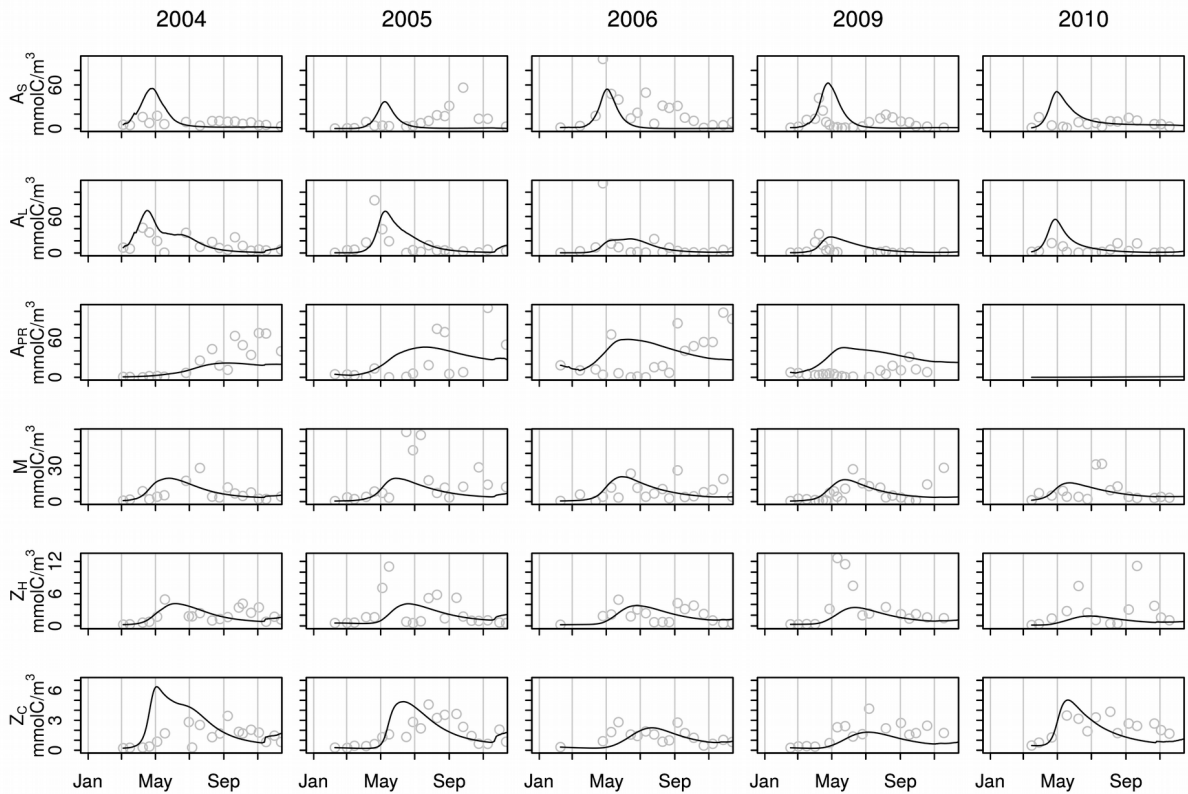
Figure 6: 0-20m averaged concentration of simulated (lines) and measured (circles) concentration of plankton groups.
