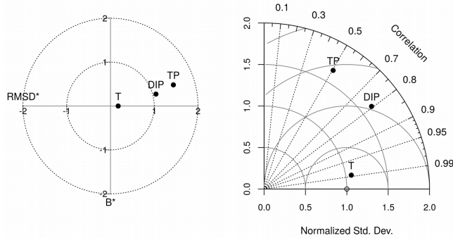
Figure 9: Target-Taylor diagrams for temperature, dissolved phosphorus and total phosphorus within the upper 80 m, depth-resolution retained, unlike in Fig.8
