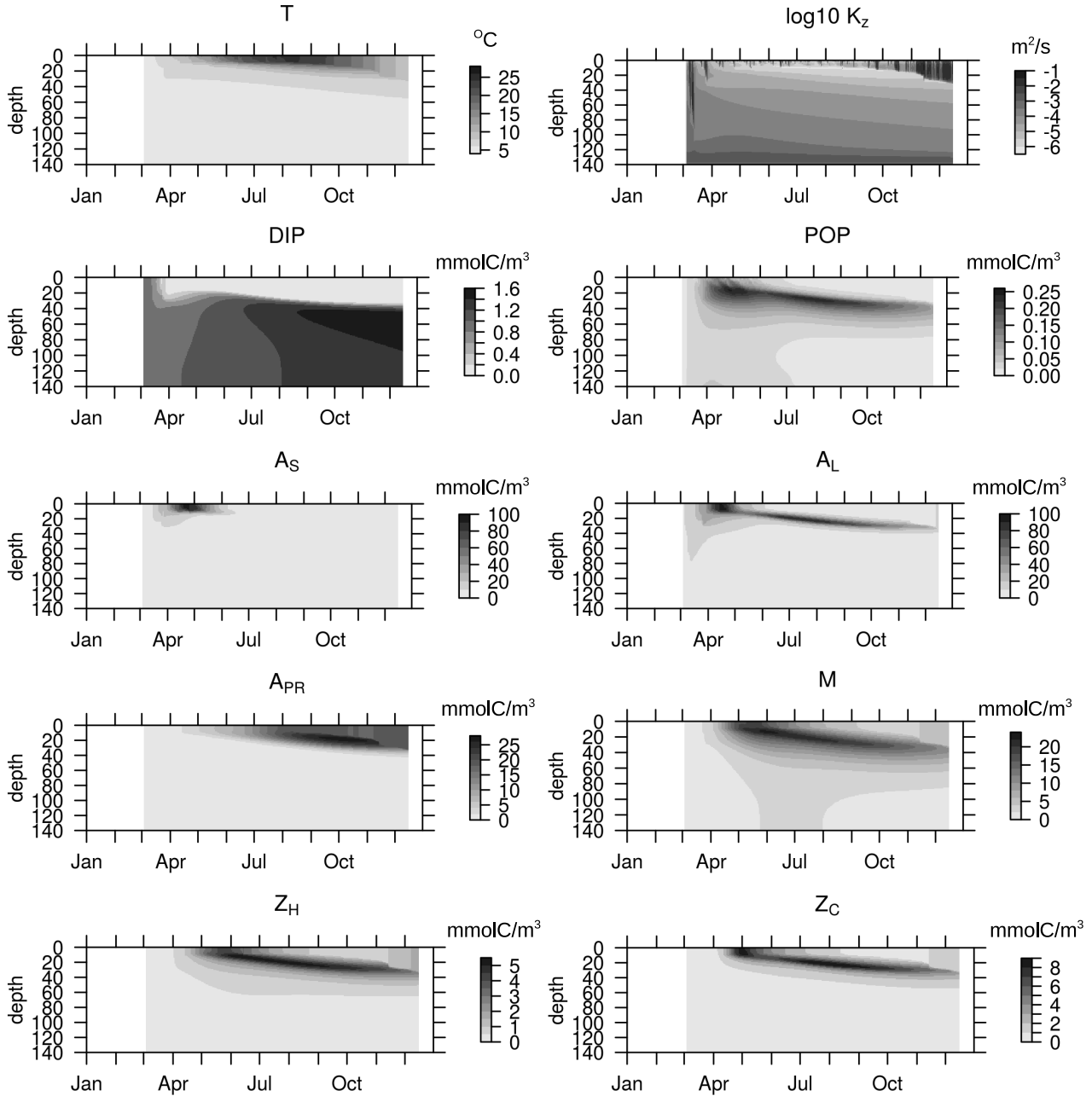
Figure 5: Spatio-temporal distribution of simulated major variables in 2004.
