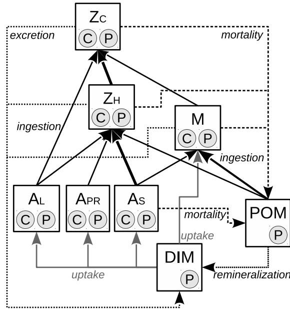
Figure 2: Model structure. DIM: dissolved inorganic matter (here phosphorus only, so referred to as DIP hereafter), POM: particulate organic matter (here phosphorus only, so referred to as POP hereafter), A_{PR} : P. rubescens , A_L : large algae, A_S : small algae, M: mixotrophs, Z_H : herbivorous zooplankton, Z_C : carnivorous zooplankton. Thick arrows indicate strong feeding preference. C and P in circles indicate carbon and phosphorus.
