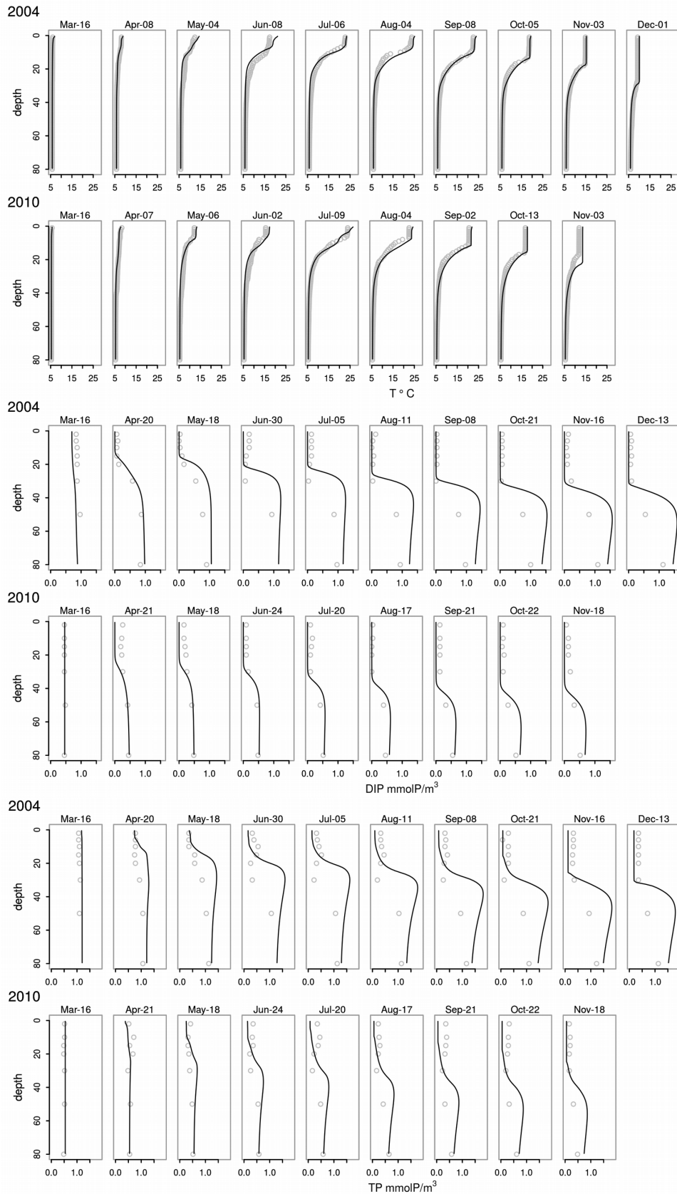
Figure 10: Simulated (lines) and measured (circles) Temperature, DIP and TP profiles from 2004 and 2010 within the upper 80 m. Only the first measurements in each month are shown. Profiles from identical months in different years are aligned.
