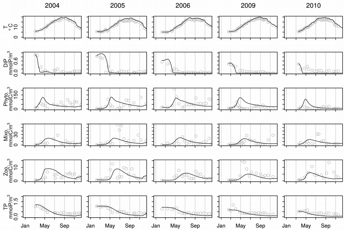
Figure 7: 0-20m averaged concentration of simulated (lines) and measured (circles) concentration of biological variables.
