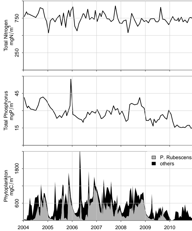
Figure 1: Observed concentrations of total phosphorus and total nitrogen (0-140 m average), and total phytoplankton and contribution by P. rubescens in Lake Bourget (0-20 m average) for the period 2004-2010.
