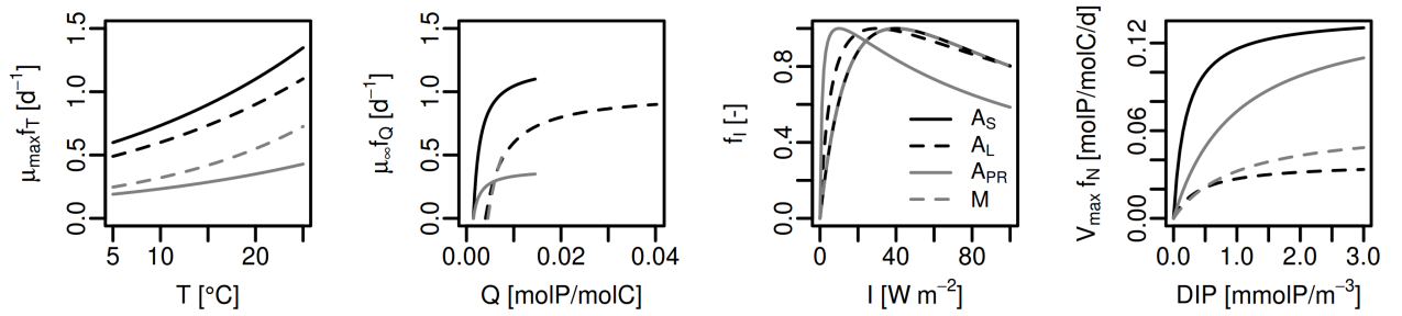
Figure 4: Limitation functions and their effects on autotrophic functions for each plankton group with the parameter values listed in Tables 3-4. f_T , f_Q , f_I and f_N stand for temperature limitation (eq. 16), nutrient limitation of biomass growth (eq. 3), light limitation of photosynthesis (eq. 5) and nutrient limitation of uptake (eq. 8), respectively.
