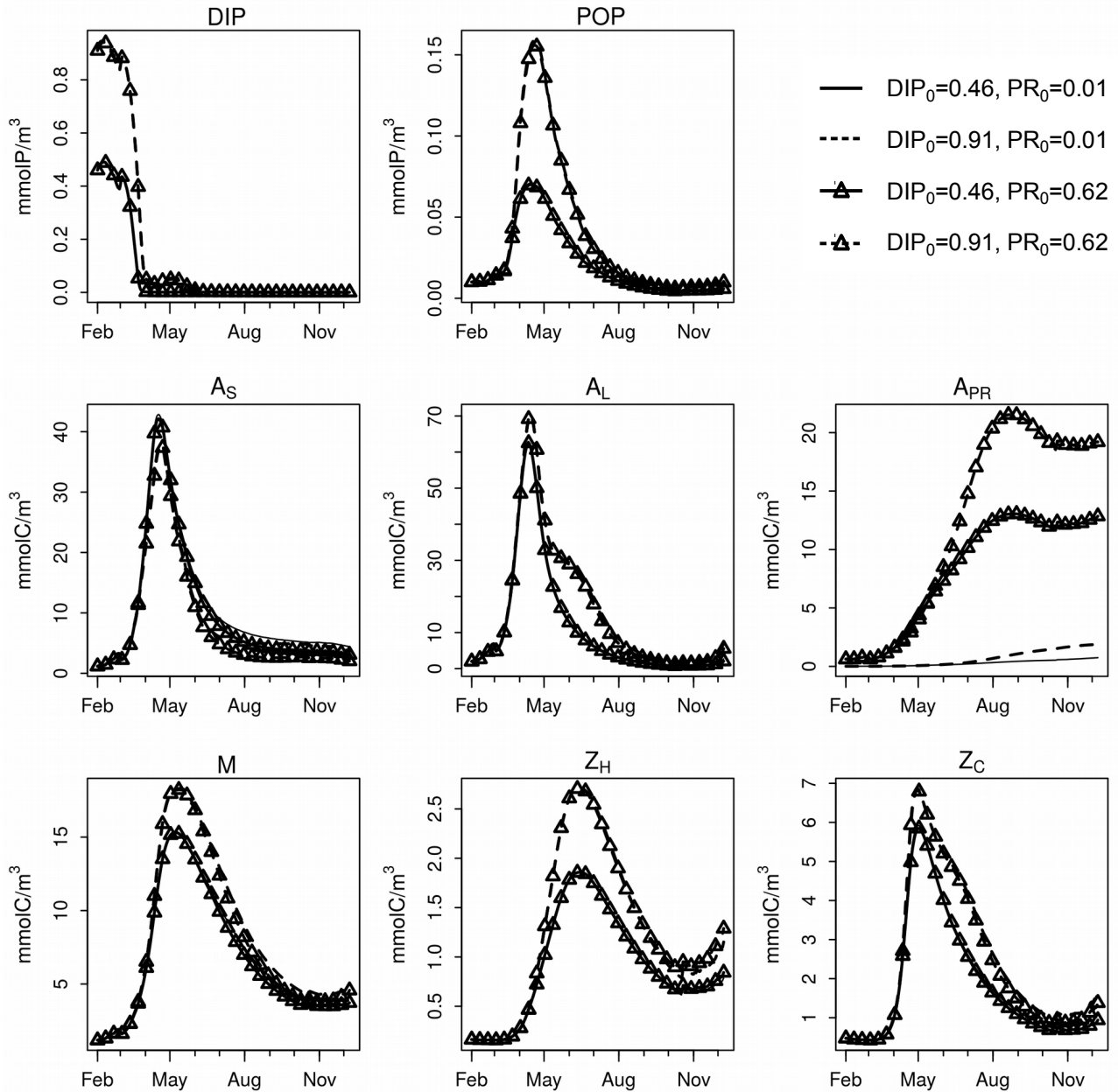
Figure 11: Surface (0-20 m) average water column average state variables with initial DIP concentration of DIP_0 = 0.46 \text{ mmolP m}^{-3} as in 2010 (solid lines), DIP_0 = 0.91 \text{ mmolP m}^{-3} as in 2004 (dashed lines), in combination with initial P. rubescens concentration of PR_0 = 0.01 \text{ mmolC m}^{-3} as (was assumed) in 2010 (no marker) and PR_0 = 0.62 \text{ mmolC m}^{-3} as in 2004 (triangles). Initial conditions for all other variables and meteorological forcing was as in 2010.
