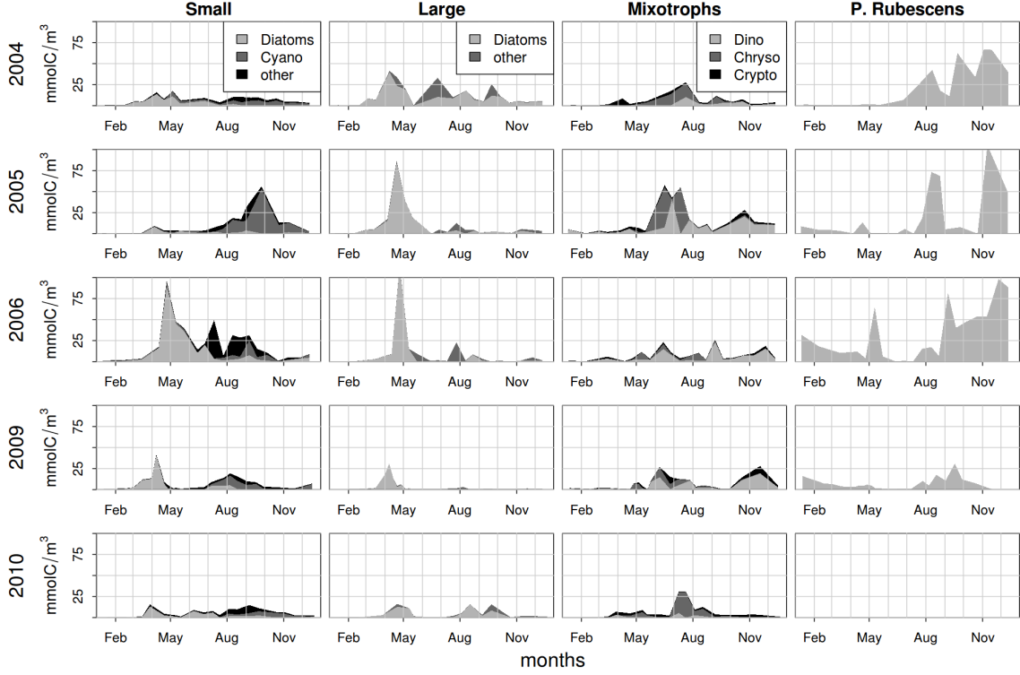
Figure 3: Measured contribution of major taxonomic classes to each phytoplankton group throughout the simulated years.
