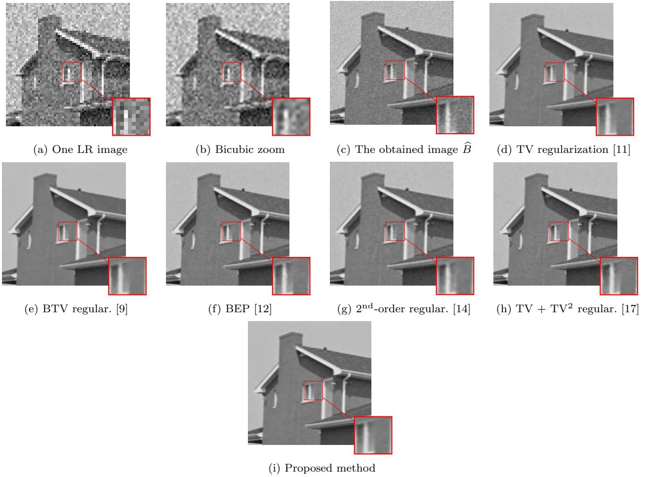
Fig. 5: Super resolution of House by different methods.
