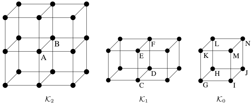
Fig. 16. \mathcal{K} -neighborhoods for 2-cliques ( \mathcal{K}_2 ), 1-cliques ( \mathcal{K}_1 ), and 0-cliques ( \mathcal{K}_0 ). A voxel is represented by its central point.
